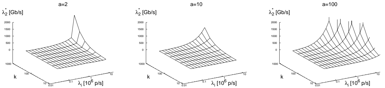
Figure 17: Traffic at the switch master port—the header passing overhead within the switch.
