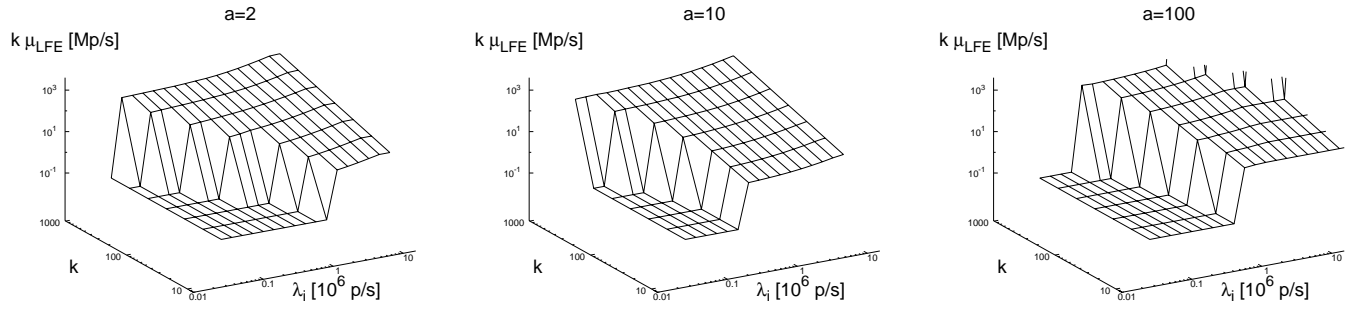
Figure 13: Total processing power of the LFEs (note that the graph was adjusted for the reader's convenience in order to be able to depict the values equal to 0, which would normally tend to negative infinity on a logarithmic graph).
