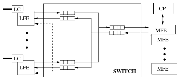
Figure 3: LFEs, switch and MFEs within the general distributed router architecture model.
