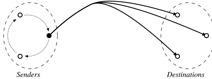
Figure 6: privilege-based algorithms.
