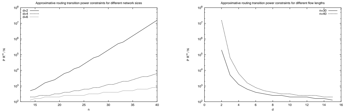
Figure 5: The two figures depict at which power constraint a transition from minimal-energy routing to direct routing occurs, as a function of n and d .
