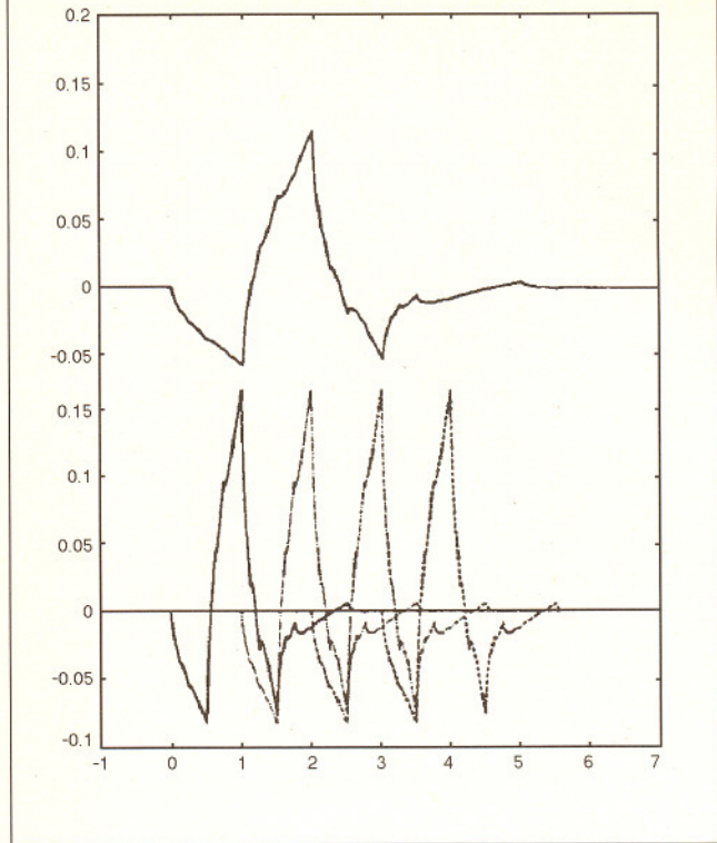
Fig. 14. Two scales of the D_4 wavelet and shifts. This set of functions is orthogonal.
