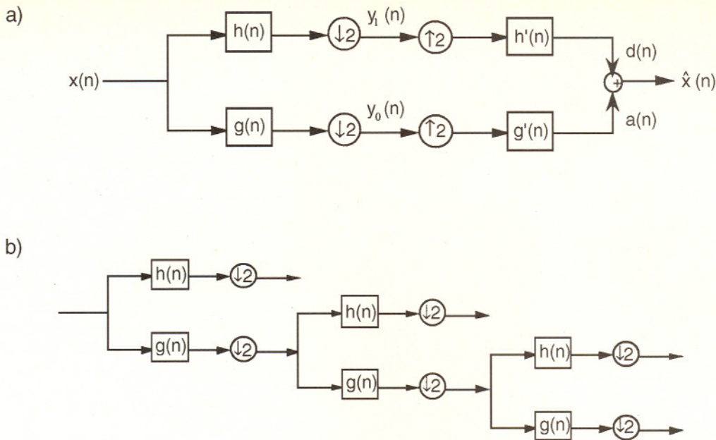
Fig. 11. Subband Coding scheme. (a) Two subsampled approximations, one corresponding to low and the other to high frequencies, are computed. The reconstructed signal is obtained by re-interpolating the approximations and summing them. The filters on the left form an analysis filter bank, while on the right is a synthesis filter bank. (b) Block diagram (Filter Bank tree) of the Discrete Wavelet Transform implemented with discrete-time filters and subsampling by two. The frequency resolution is given in Fig. 3b.
