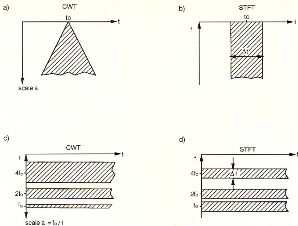
Fig. 4. Regions of influence of a Dirac pulse at t=t_0 (a) for the CWT and (b) for the STFT; as well as of three sinusoids (of frequencies f_0 , 2f_0 , 4f_0 ) for (c) the CWT and (d) the STFT.
