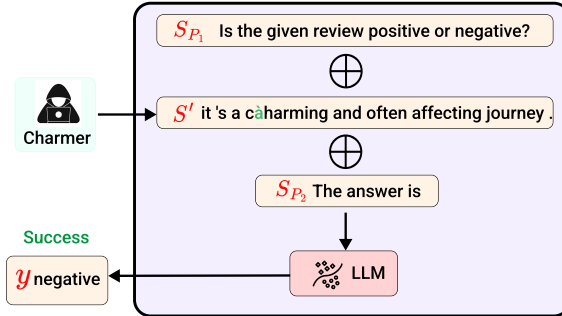
Figure S6. Schematic of the proposed Charmer in attacking LLM-classifiers. Charmer modifies the input to S' with a small perturbation (annotated in green color) to the original input so that the model produces the desired output y . S_{P_1} and S_{P_2} are auxiliary prompts that remain unchanged during the attack.
