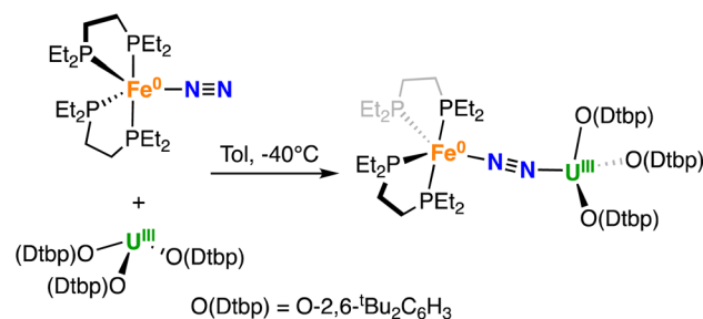
Scheme 2 Synthesis of 2 .
