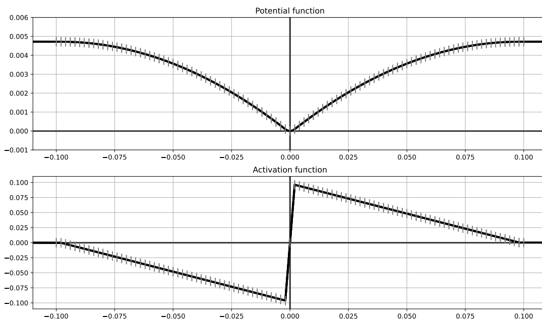
Figure 3.5. Potential function \psi and activation function \varphi = \psi' of the learned WCRN-NN. These functions are splines of degrees 2 and 1, respectively. The vertical markers indicate the control points of the splines.
