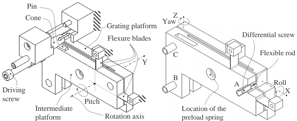
FIGURE 2. Sketches of the 4 degrees-of-freedom flexure-based unit. Left: Pitch Module. Right: Yaw-Roll-Y Module (the drawing of the differential screw is simplified for clarity).
