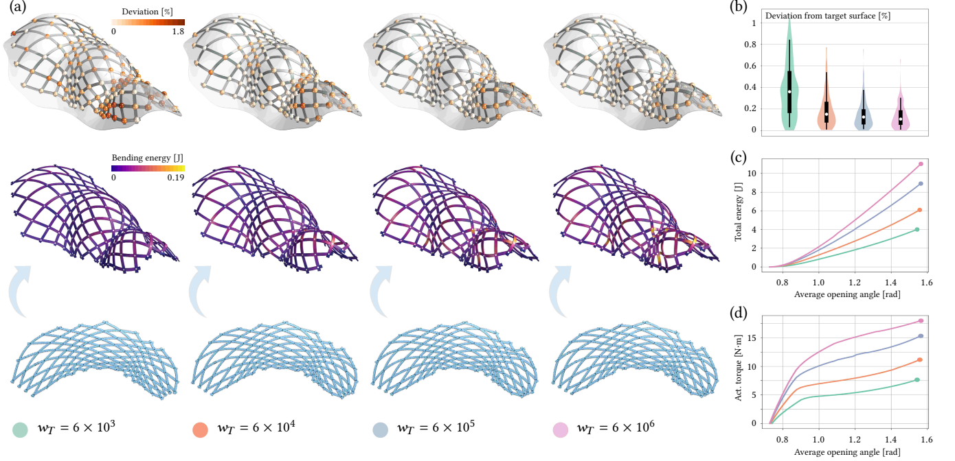
Fig. 5. (a) The surface fitting weight w_T controls the tradeoff between target fitting (top) and elastic energy (middle). Deviation to the target surface is reported as a percentage of the diagonal of the surface’s bounding box. (b) Target surface fitting histograms measure the deviation from the target surface. White dots represent the medians, thick lines show the inter-quartiles, and thin lines indicate the 5th to 95th percentile range. (c) The total energy at a certain opening angle, (d) corresponding torque required to hold the structure.
