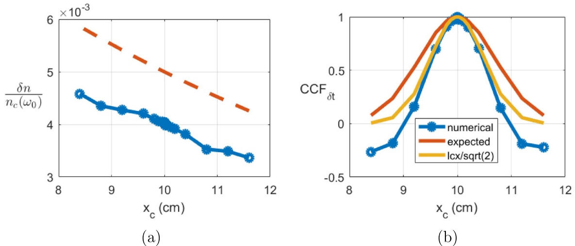
Figure 17. Exponential \delta n(x) amplitude profile case. (a) Turbulence amplitude profile computed according to equation (17). The blue curve corresponds to the full-wave computation data, the red dashed line corresponds to the turbulence amplitude profile used as input. (b) Delay CCF function. The blue curve corresponds to the full-wave computation, the red curve corresponds to the input Gaussian turbulence CCF and the yellow curve corresponds to the same dependence with l_{cx} divided by \sqrt{2} .
