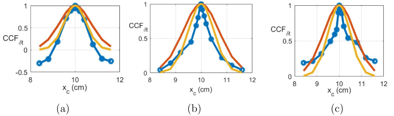
Figure 21. Delay CCF function for relative turbulence amplitude \delta n/n_c(\omega_0) (a) 0.0017, (b) 0.058 and (c) 0.13. The Blue curves correspond to the full-wave computation, the red curves correspond to the input Gaussian turbulence CCF and the yellow curves correspond to the Gaussian dependence with l_{cx} divided by \sqrt{2} .
