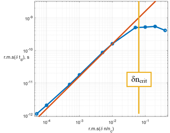
Figure 10. R.m.s of X-mode time delay vs the amplitude of the turbulence in the 1D limit. The blue curve corresponds to the full-wave computation, the red line is the prediction given by equation (15) multiplied by a factor of 2. The yellow line is the threshold amplitude given by equation (14).
