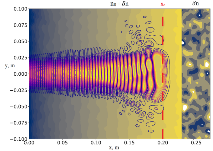
Figure 8. An example of the CUWA computation. The filled contours correspond to the full density profile n_0 + \delta n (on the left, for x < 0.225 m) and its perturbation \delta n (on the right, for x > 0.225 m). The blue contour lines correspond to the electric field.
