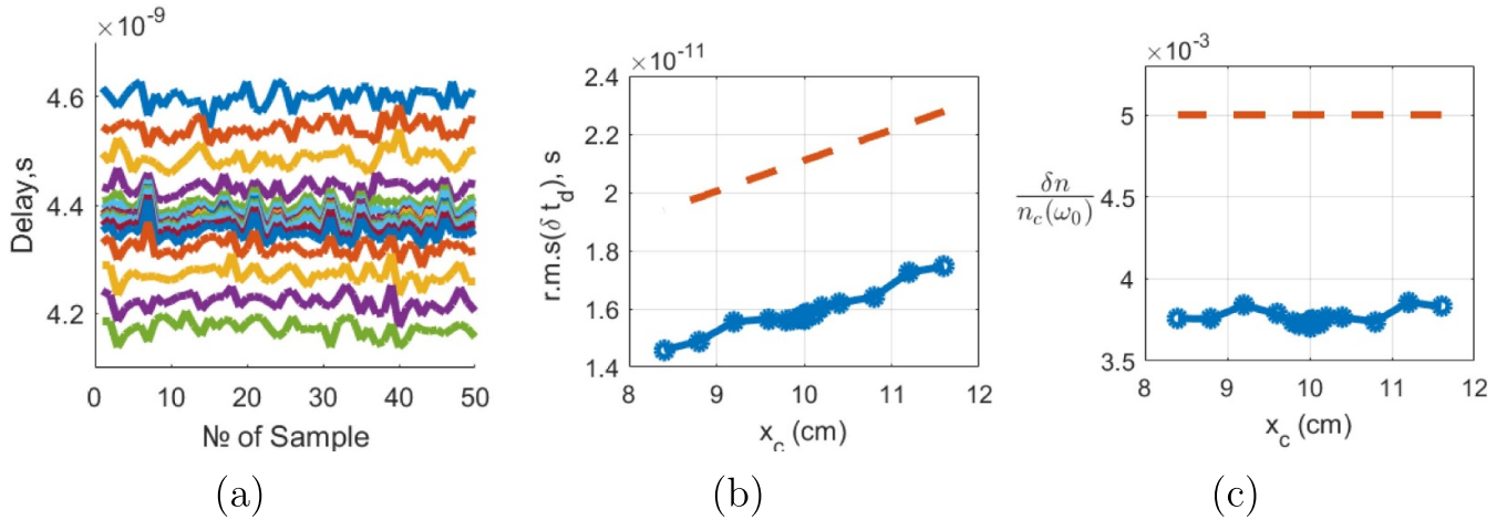
Figure 14. Example of data analysis process. (a) Delays computed for each turbulence sample (different colours correspond to different probing frequencies); (b) r.m.s. of delays computed for each probing frequency vs the cut-off radial position. The blue curve corresponds to the full-wave computation and the red dashed line is the prediction given by equation (17); (c) turbulence amplitude profile. The blue curve corresponds to the full-wave computation data, the red dashed line corresponds to the constant turbulence amplitude profile used as an input for the full-wave computation.
