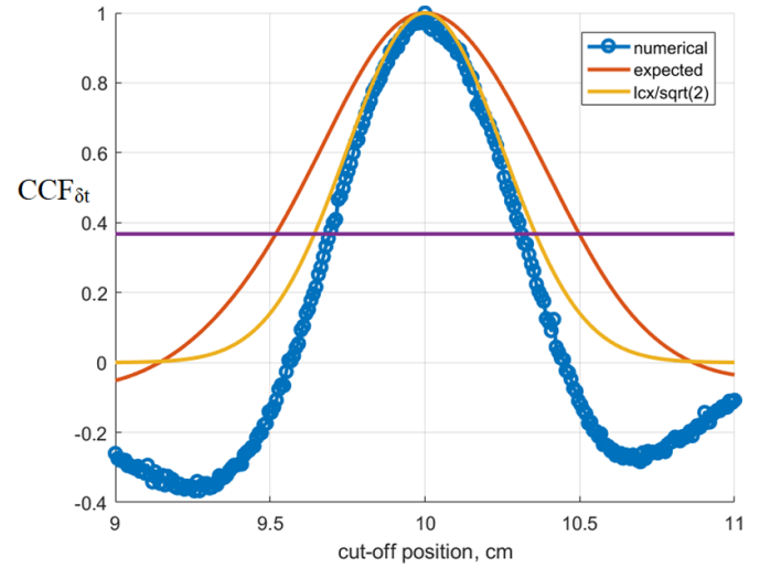
Figure 6. CCF of O-mode time delays corresponding to different cut-off positions for L = 10 cm and l_{cx} = 0.5 cm. The blue curve corresponds to the numerical integration, the red line is the prediction given by equation (13). The yellow line is the same formula with l_{cx} divided by \sqrt{2} . The purple line corresponds to 1/e level.
