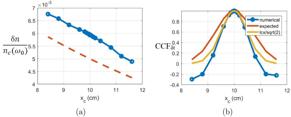
Figure 18. 1D \delta n case. (a) Turbulence amplitude profile computed according to equation (17). The blue curve corresponds to the full-wave computation data, the red dashed line corresponds to the turbulence amplitude profile used as input. (b) Delay CCF function. The blue curve corresponds to the full-wave computation, the red curve corresponds to the input Gaussian turbulence CCF and the yellow curve corresponds to the same dependence with l_{cx} divided by \sqrt{2} .
