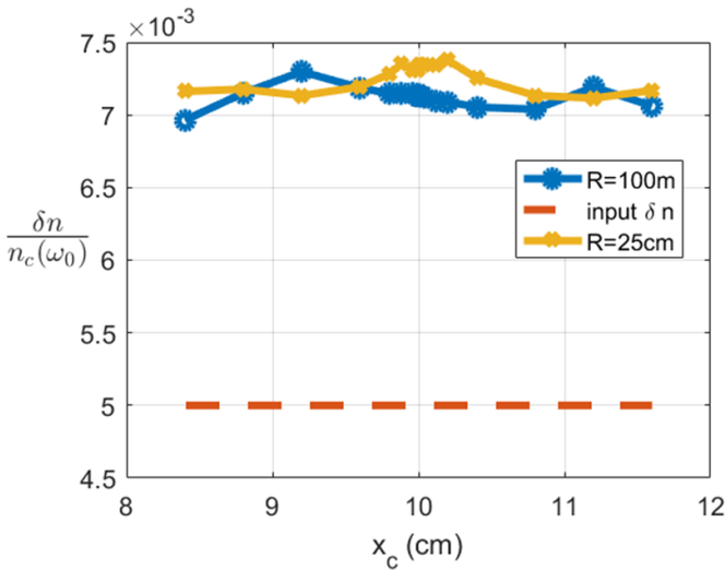
Figure 20. Turbulence amplitude profile computed according to equation (17). The blue and yellow curves correspond to the full-wave computation data considering l_{cy} = 20 cm as well as R = 100 m and R = 25 cm respectively, the red dashed line corresponds to the profile used as input for the full-wave computation.
