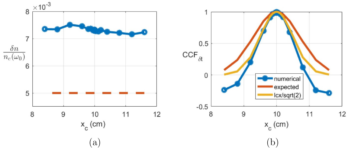
Figure 19. Finite plasma curvature case. (a) Turbulence amplitude profile computed according to equation (17). The blue curve corresponds to the full-wave computation data, the red dashed line corresponds to the turbulence amplitude profile used as input. (b) Delay CCF function. The blue curve corresponds to the full-wave computation, the red curve corresponds to the input Gaussian turbulence CCF and the yellow curve corresponds to the same dependence with l_{cx} divided by \sqrt{2} .
