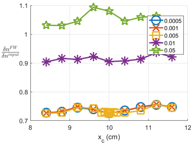
Figure 15. Turbulence amplitude profile normalised to input amplitudes. Different colours and markers correspond to different values of the relative input amplitude at the central cut-off.
