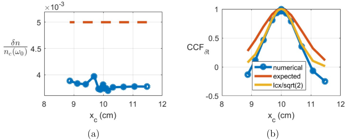
Figure 16. Quadratic n_0(x) profile case. (a) Turbulence amplitude profile computed according to equation (17) with input l_{cx} value. The blue curve corresponds to the full-wave computation data, the red dashed line corresponds to the turbulence amplitude profile used as input. (b) Delay CCF function. The blue curve corresponds to the full-wave computation, the red curve corresponds to the input Gaussian turbulence CCF and the yellow curve corresponds to the same dependence with l_{cx} divided by \sqrt{2} .
