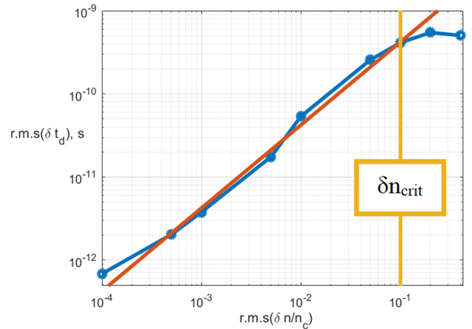
Figure 11. R.m.s of O-mode time delay vs the amplitude of the turbulence for realistic parameters. The blue curve corresponds to the full-wave computation, the red line is the prediction given by equation (17). The yellow line is the threshold amplitude given by equation (6).
