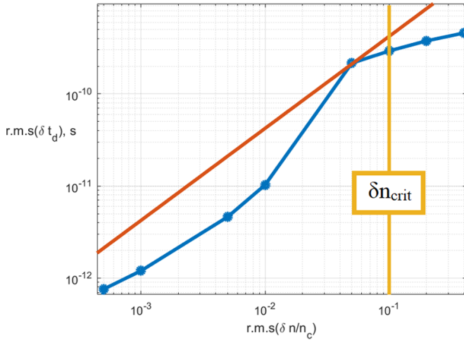
Figure 12. R.m.s of O-mode time delay vs the amplitude of the turbulence for large relative beam waist \rho/l_{cy} . The blue curve corresponds to the full-wave computation, the red line is the prediction given by equation (17). The yellow line is the threshold amplitude given by equation (6).
