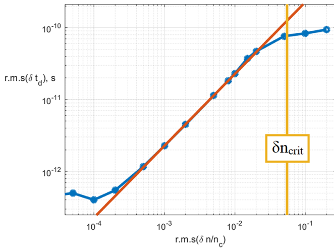
Figure 5. Numerical integration example for L = 4 cm and l_{cx} = 0.22 cm. R.m.s. of O-mode time delay vs the amplitude of the turbulence. The blue curve corresponds to the numerical integration, the red line is the prediction given by equation (10), multiplied by 2. The yellow line is the threshold amplitude given by equation (6).
