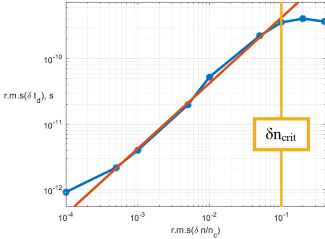
Figure 9. R.m.s of O-mode time delay vs the amplitude of the turbulence in the 1D limit. The blue curve corresponds to the full-wave computation, the red line is the prediction given by equation (17). The yellow line is the threshold amplitude given by equation (6).
