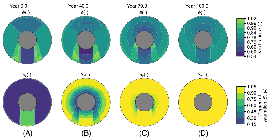
FIGURE 21 Evolution of the spatial distribution of the void ratio and degree of saturation in the initially segregated buffer case. (A) Initial state. (B) After 40 years. (C) After 70 years. (D) After 100 years.
