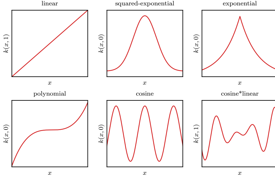
Figure 2.1: Examples of positive-definite kernels.
