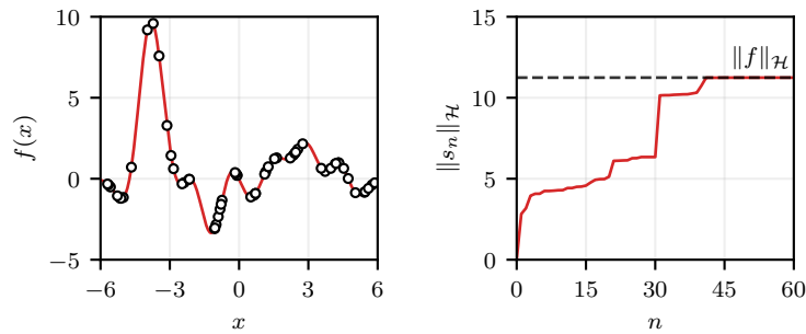
Figure 2.14: Estimating the RKHS norm of a function (left) from samples. The norm value of the MNI interpolant for an increasing number of samples (right) is shown to gradually approach the RKHS norm of the ground-truth.
