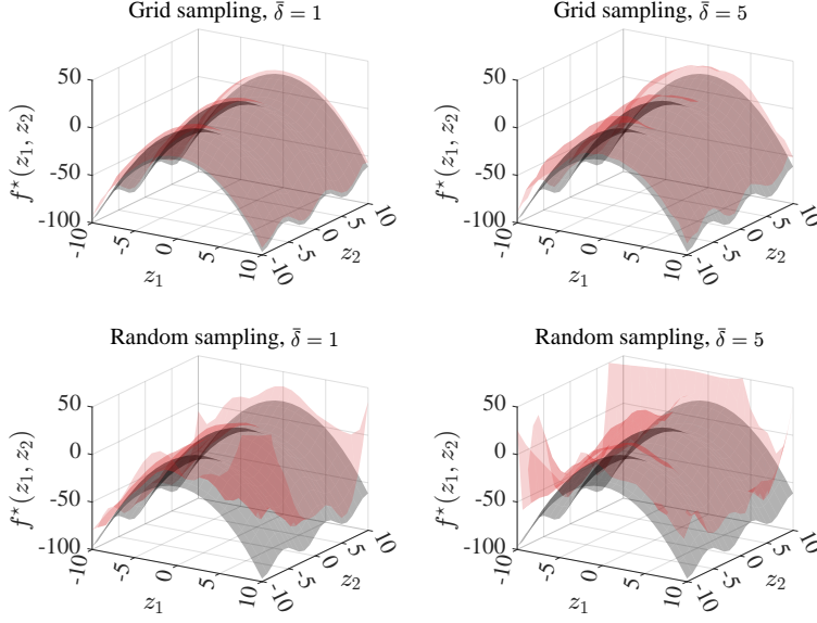
Figure 2.8: The ground-truth (black) and the optimal upper bound C(x) (red) with 100 data-points and different sampling methods and noise levels.
