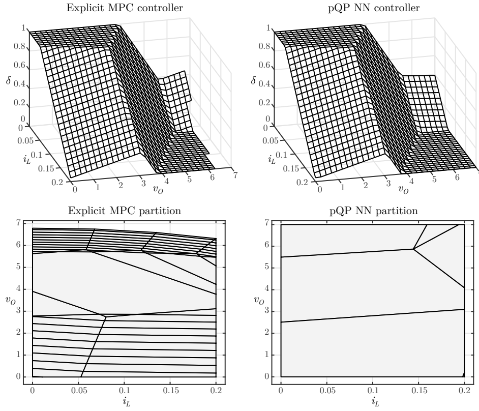
Figure 4.7: The original explicit MPC map and its domain partition (left), and the learned pQP NN map and its domain partition (right).
