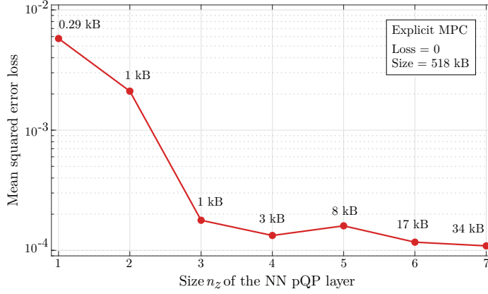
Figure 4.3: Neural network training loss as a function of the pQP layer size, and storage requirements associated with their PWA representations.
