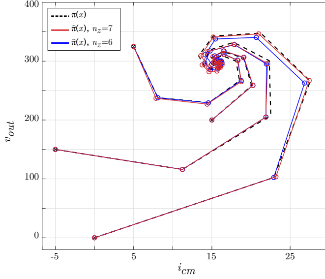
Figure 4.5: Output voltage and common mode current phase portraits under the explicit MPC controller and the two viable pQP NN approximations.
