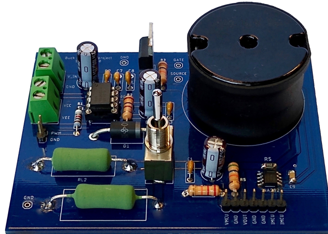
Figure 4.8: A picture of the Buck converter prototype designed and assembled in the Automatic Control Laboratory at EPFL.
