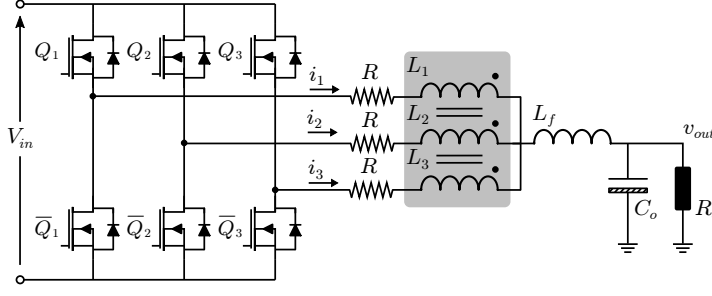
Figure 4.2: A diagram of the multi-cell step-down DC-DC converter.
