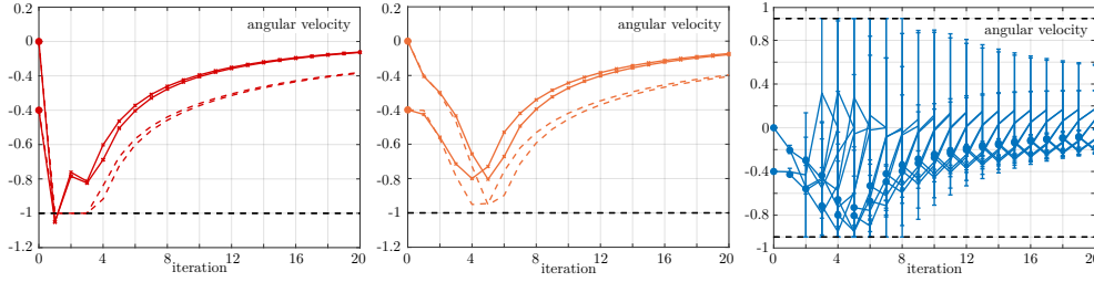
Figure 2.13: Left: Nominal kernel-MPC predictions (dashed) and closed-loop trajectory (solid). Center: KPC predictions (dashed) and closed-loop trajectory (solid). Right: KPC full open-loop predictions, confidence intervals, and initial points depicted as circular markers.
