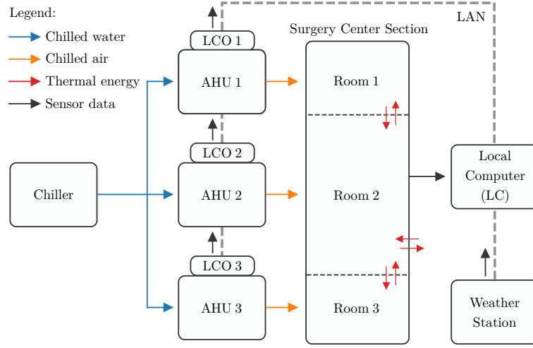
Figure 3.4: The overall system architecture, including the three AHUs and their local controllers (LCOs). Information is exchanged between the LCOs and the local computer (LC) through a local area network (LAN).
