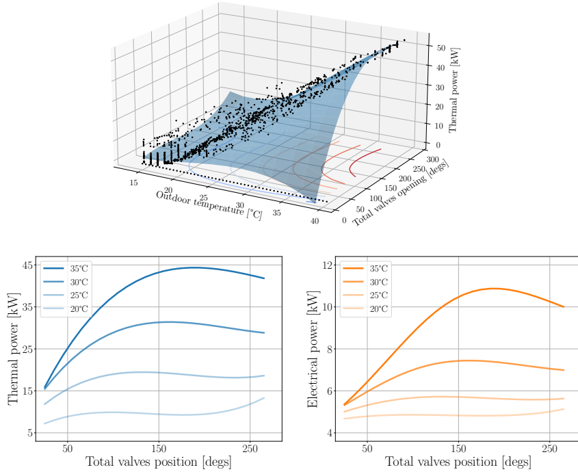
Figure 3.6: Reconstruction of the chiller refrigeration surface (top). Data were collected during a period of 203 hours, including both of open-loop excitation as well as closed-loop operation. Thermal power Q(T_{\text{out}}, \Theta) (bottom left) and electrical power E(T_{\text{out}}, \Theta) (bottom right) curves of the chiller as a function of the valves openings \Theta . The plots consider typical outdoor temperature values.
