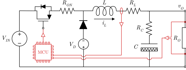
Figure 4.6: A circuit diagram of the Buck converter including its parasitic resistances and the diode forward voltage drop. The feedback loop is closed by the microcontroller that implements our proposed pQP NN scheme.
