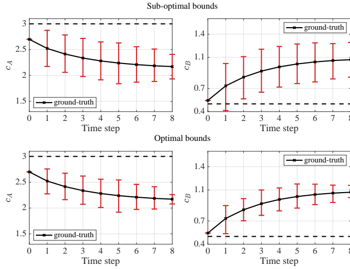
Figure 2.12: State trajectories of the CSTR system under the same control inputs, but with different uncertainty quantification techniques. Constraints are represented by the dashed lines.
