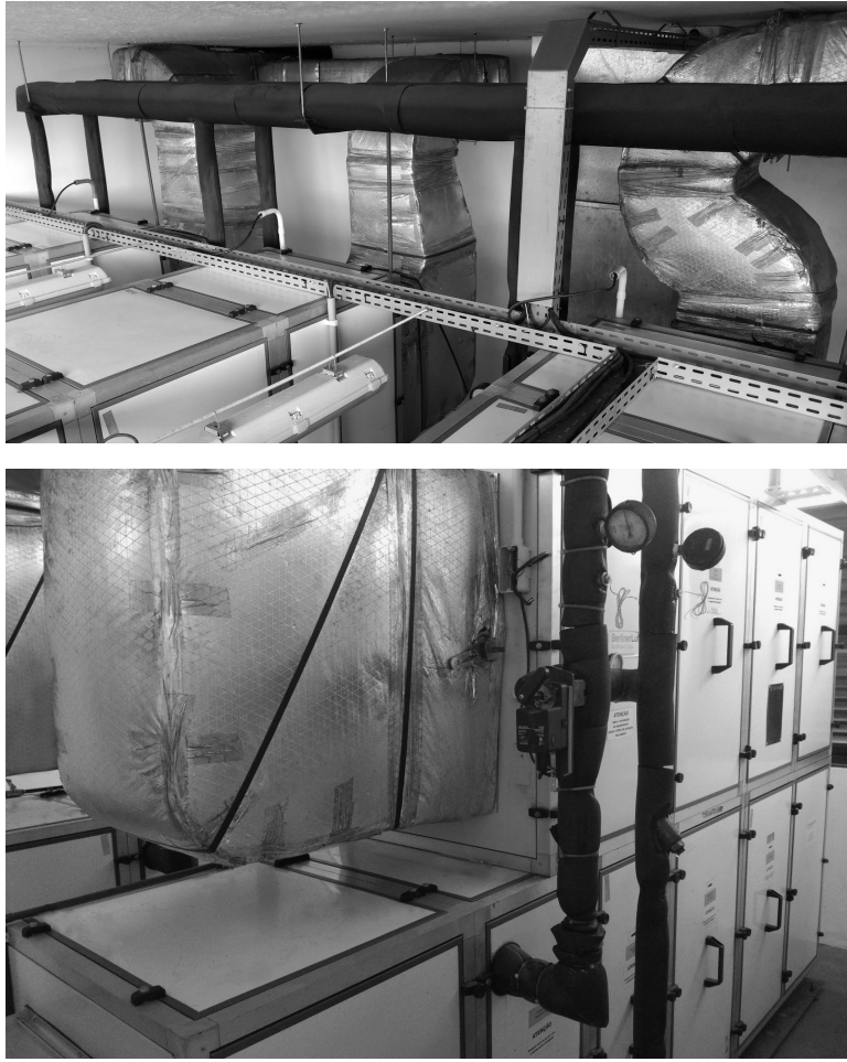
Figure 3.3: Photos of the AHU room where one can identify the air ducts (top), the supply and return water pipes (top and bottom), and one of the three-way valve servomotors that control the flow of chilled water (bottom).
