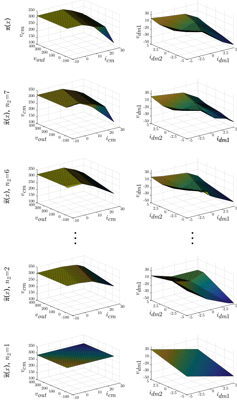
Figure 4.4: Slices of the explicit MPC controller \pi(x) and the pQP NN approximations \hat{\pi}(x) for two control variables: v_{cm} (left) and v_{dm1} (right).
