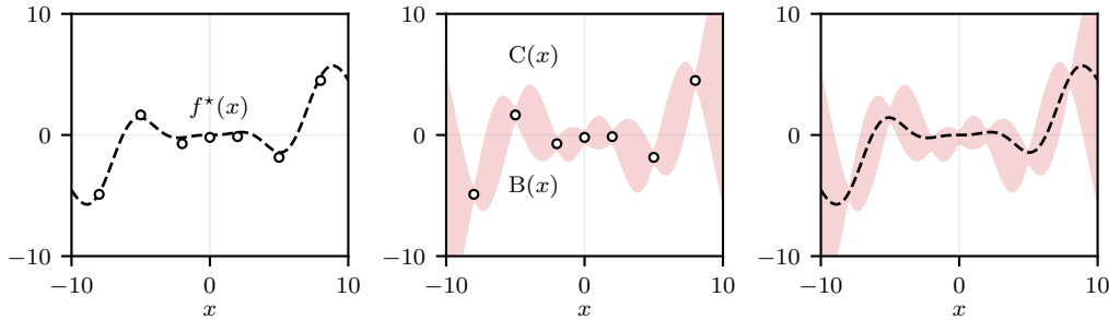
Figure 2.3: Optimal bounds example for the SE kernel (2.3) with \ell = 2.5 . Left: a member f \in \mathcal{H} with \|f\|_{\mathcal{H}} = 16.42 and 7 data-points with \bar{\delta} = 0.5 . Center: data-points and the optimal bounds C(x) , B(x) computed with \Gamma = 1.1 \|f\|_{\mathcal{H}} . Right: the ground-truth f(x) and the optimal bounds C(x) , B(x) .
