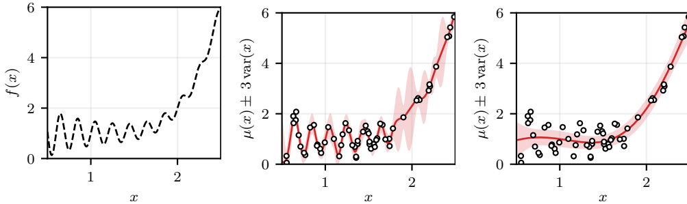
Figure 3.1: A Gaussian process regression example. The ground-truth (left), Gaussian process mean and the 3\sigma confidence interval for a model with log marginal likelihood \mathcal{L} = -29.8 (middle) and \mathcal{L} = -48.5 (right).
