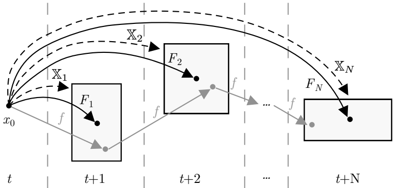
Figure 2.7: The outcome of each map: Nominal predictions F_t (—), confidence sets \mathbb{X}_t (- -), and the unknown ground-truth f (—). All functions also depend on the chosen control sequence, which is omitted for clarity.
