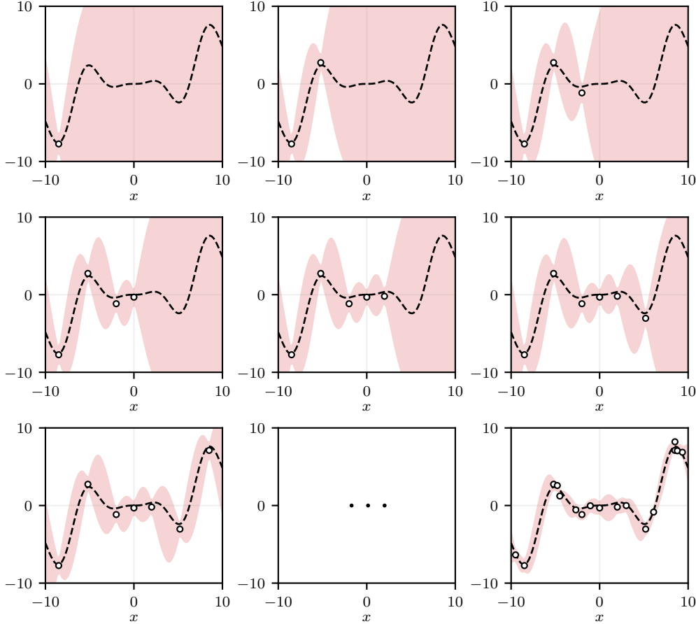
Figure 2.5: Adding new samples to a dataset can only cause uncertainty to be reduced everywhere in the domain. The noise was drawn from a uniform distribution bounded in absolute value by \bar{\delta} = 0.8 . The last plot depicts the bounds after the collection of 10 new random samples.
