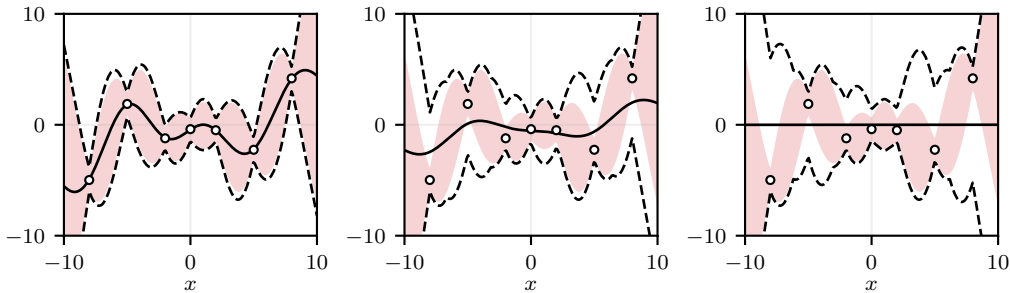
Figure 2.6: A comparison between the optimal bounds (red envelopes) and the closed-form sub-optimal bounds (dashed black lines) around KRR models (solid black lines). Three KRR distinct regularization constants were tested \lambda = 10^{-3} (left), \lambda = 10^{-1} (center) and \lambda = 10^2 (right).
