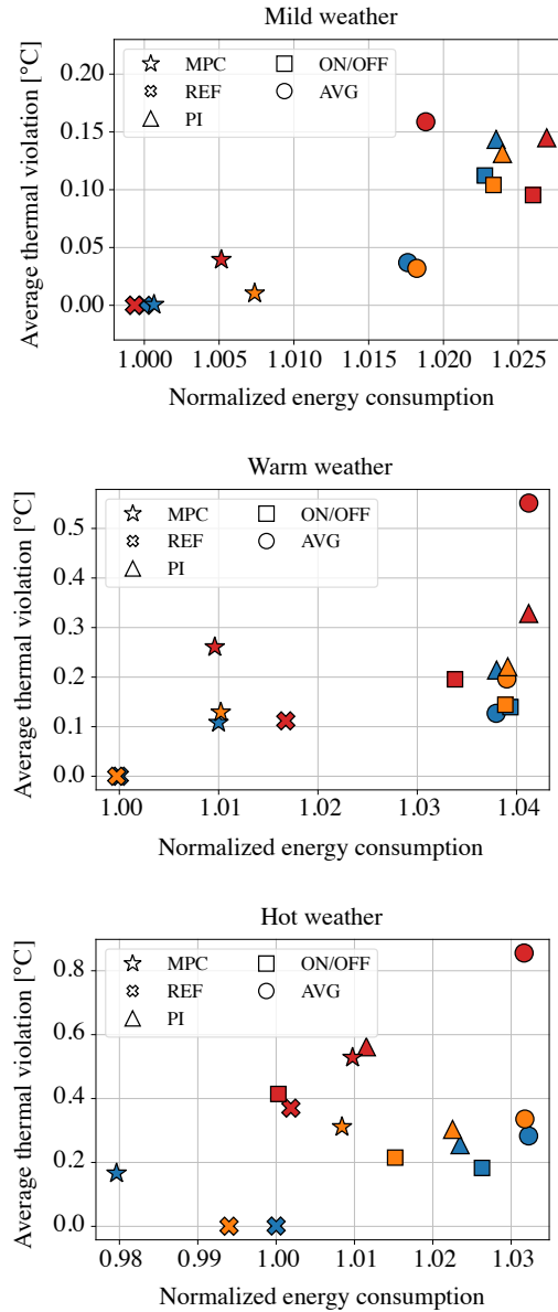
Figure 3.9: Simulation results of the normalized energy consumption and thermal performance (average temperature bound violation) of different control strategies. Three weather profiles were considered: mild, warm and hot. The indoor temperatures were initialized at three different values according to the color scheme: 17°C (blue), 19°C (orange) and 21°C (red).
