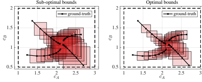
Figure 2.11: Phase portraits of the CSTR system under the same control inputs, but with different uncertainty quantification techniques. Constraints are represented by the dashed lines.
