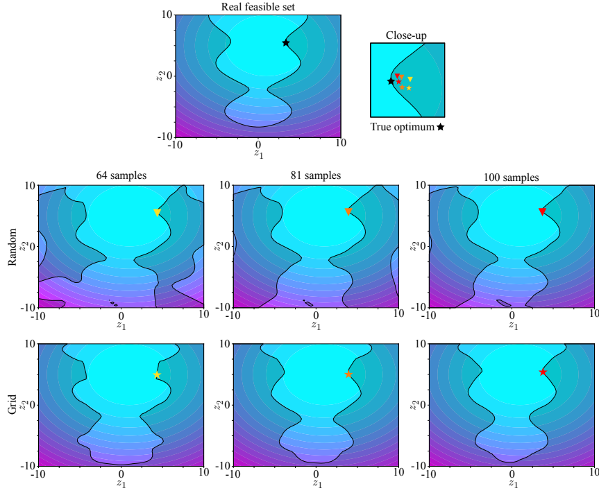
Figure 2.10: Solutions and feasible sets (shaded areas) of the surrogate optimization problems, i.e., (2.41) with the constraint replaced by its optimal upper bound C(x) \leq -10 . The individual solutions are denoted by the yellow, orange and red triangles and stars. The true optimum is indicated by a black star.
