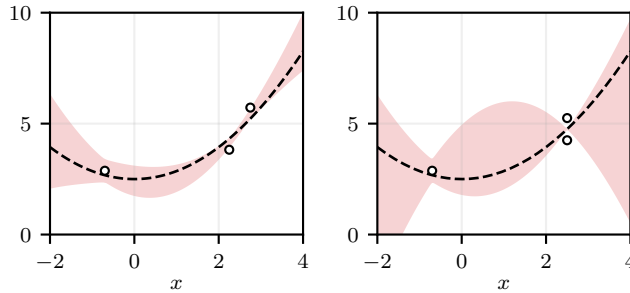
Figure 2.4: Left: samples lying outside of the uncertainty envelope, implying that its width is smaller than \bar{\delta} at those locations. Right: redundant information is used to shrink the uncertainty envelope and recover the exact ground-truth value at x = 2.5 as C(2.5) = B(2.5) = f^*(2.5) = 4.75 .
