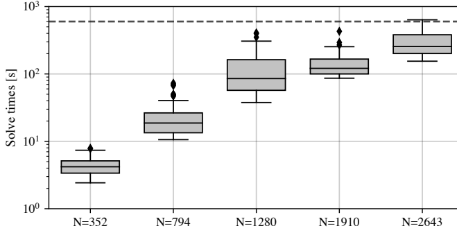
Figure 3.7: Box and whisker plots of the MPC solve times considering different dataset sizes. The dashed gray line marks our sampling period of 10 mins. Each boxplot is based on 50 time samples, obtained using randomized initial conditions.
