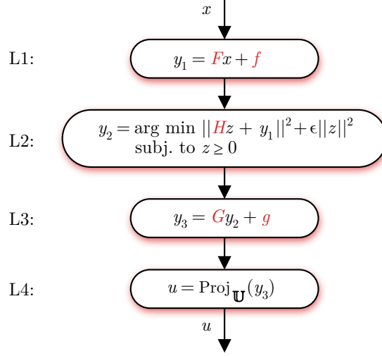
Figure 4.1: A pQP neural network architecture tailored to MPC. The variables in red are weights to be adjusted during training.
