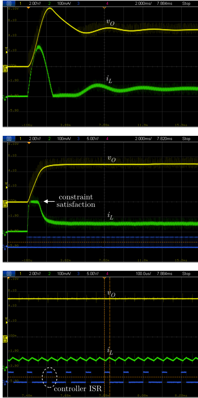
Figure 4.9: Open-loop start-up response (top), closed-loop start-up response (middle), and a close-up view of the closed-loop start-up response highlighting individual switching cycles and the controller interrupt service routine (ISR) execution time of approximately 27 \mu\text{s} .
