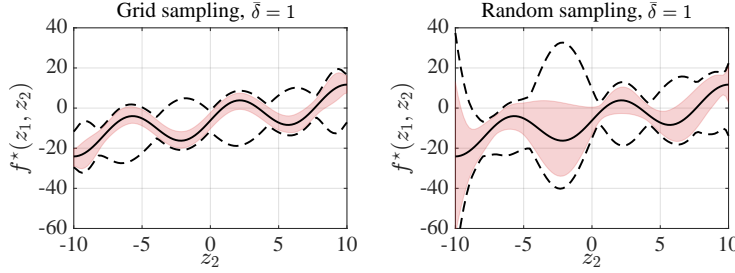
Figure 2.9: The ground-truth (solid black) sliced at z_1 = -3 , the optimal bounds (red) and the sub-optimal bounds (dashed black).
