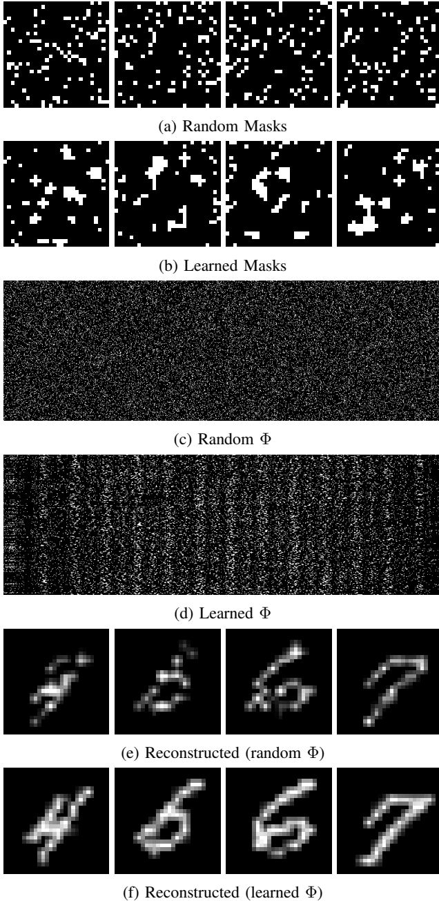
Fig. 4: Single pixel imaging masks for m = 250 , where d = 90 ones per row are selected (i.e., ones per mask). The reconstructions are obtained by T = 20 IHT-iterations.
