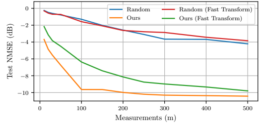
Fig. 11: Comparing the NMSE on the MNIST test set of fast-transformable single pixel imaging matrices with d = 32 to regular single pixel imaging using IHT with T = 15 iterations.
