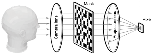
Fig. 1: Schematic visualization of a single-pixel imaging setup; image adapted from [51].
