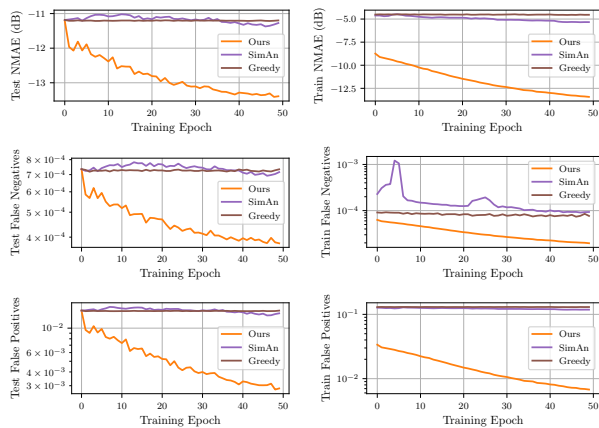
Fig. 15: NMAE (top), false negatives (middle) and false positive (bottom) at training time with T = 200 iterations (right) and during inference with T = 1000 iterations (left) of the unrolled NNLAD algorithm. Despite the train/test mismatch, GLODISMO is able to learn a \Phi that outperforms the baselines.
