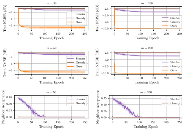
Fig. 10: Comparing the test NMSE (top), train NMSE (middle) and the average neighbor acceptance rate of the baseline algorithms throughout a training epoch (bottom) in the single pixel imaging setup from Section IV with m = 50 (left) and m = 200 (right) measurements. The shaded area represents the standard deviation over 10 random seeds. This figure highlights the training stability of GLODISMO and shows that it is not overly dependent on the random seed. Furthermore, the bottom plots show that the baselines are reasonably tuned.
