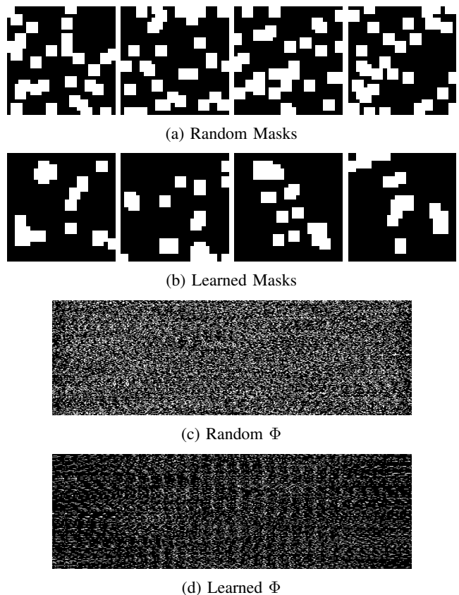
Fig. 14: Super-pixel masks for single pixel imaging with d = 32 super-pixels per mask. The masks of the learned \Phi clearly exhibit structure adapted to the MNIST dataset.
