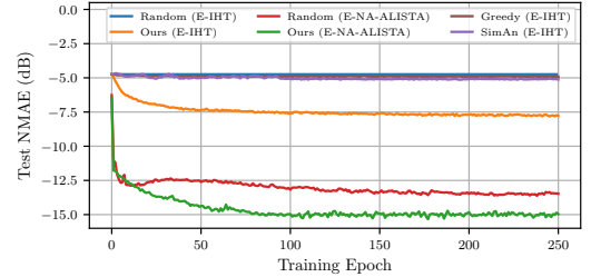
Fig. 6: NMAE of compressed sensing with left- d -regular graphs on synthetic data as a function of the training progress.
