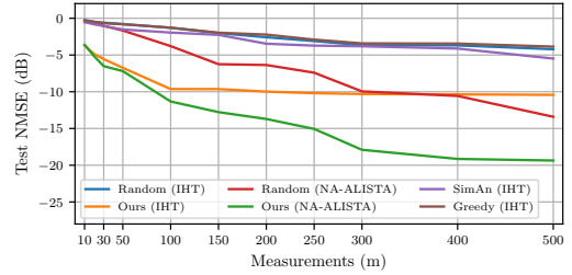
Fig. 2: NMSE of reconstruction with single pixel imaging masks as a function of the number of measurements m .
