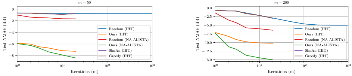
Fig. 3: NMSE of image reconstruction with single pixel imaging masks as a function of the number of iterations t for m = 50 (left) and m = 200 measurements (right).
