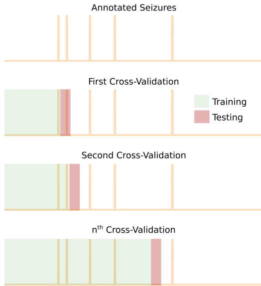
Figure 2. Proposed time-series cross-validation approach.
