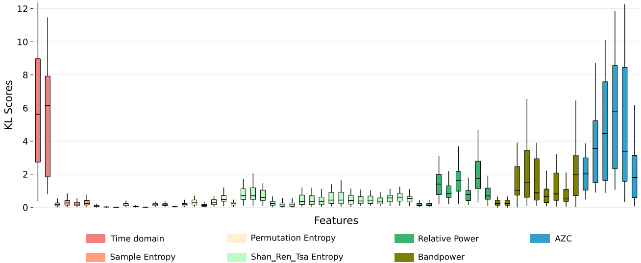
Figure 3. KL divergence scores distribution, per feature, for the CHB-MIT dataset. For a detailed description of the features, please refer to Section 3.5.
