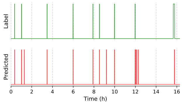
Figure 7. AZC prediction for CHB-MIT subject chb24 .
