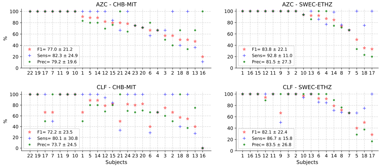
Figure 4. Performance metrics obtained with AZC-/CLF-based classification approaches, on both datasets.
