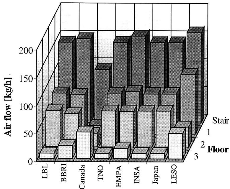
Figure 5 Comparison between the zonal air flows obtained by various participants to first run of user test 1
