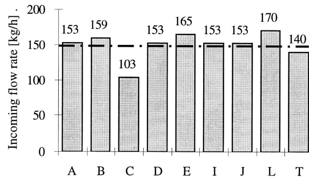
Figure 6: Comparison of total air flow rates into the building. Second run on user test 1.
