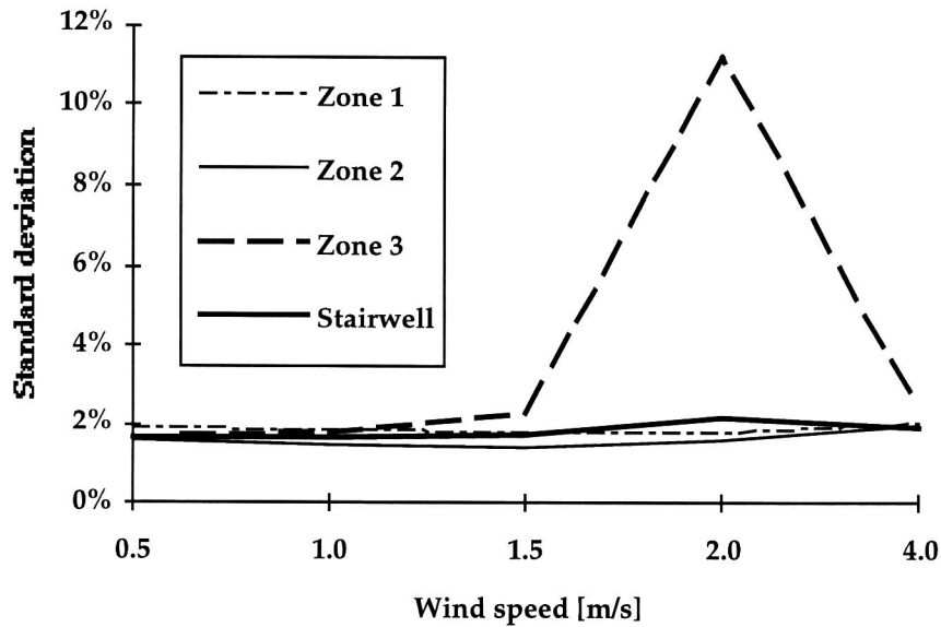
Figure 2: Variation of the standard deviation \sigma for the mean age of air obtained with 256 simulations.
