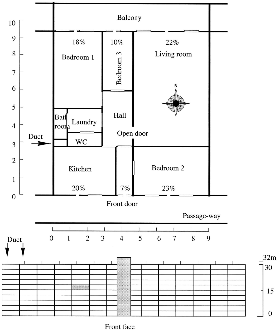
Figure 8: User test 2 building.
