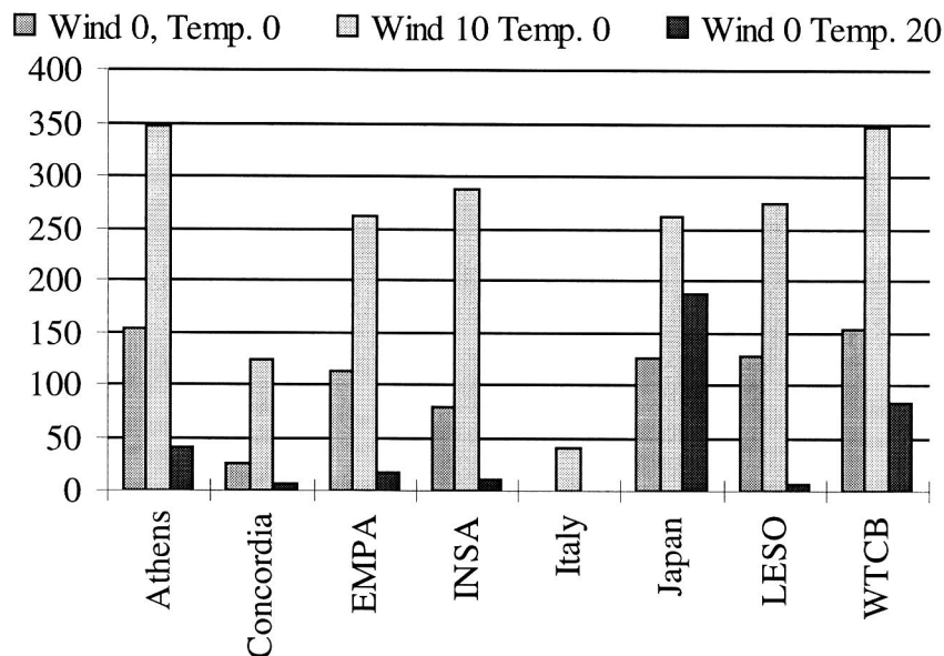
Figure 9: Total outdoor air flow rate as calculated by participants for three different conditions.
