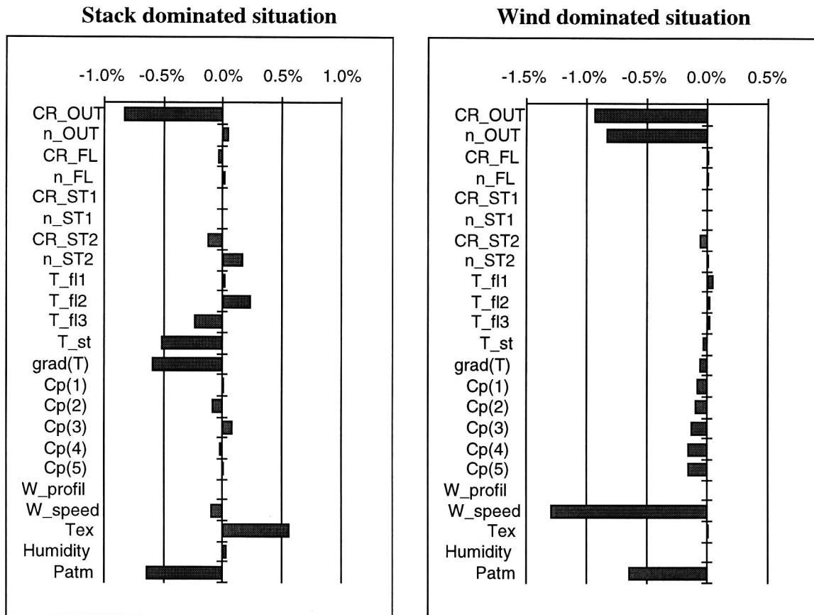
Figure 4: Comparison of main effects in a stack dominated situation ( W_{speed} = 1m/s ) and a wind dominated one ( W_{speed} = 4m/s ).
