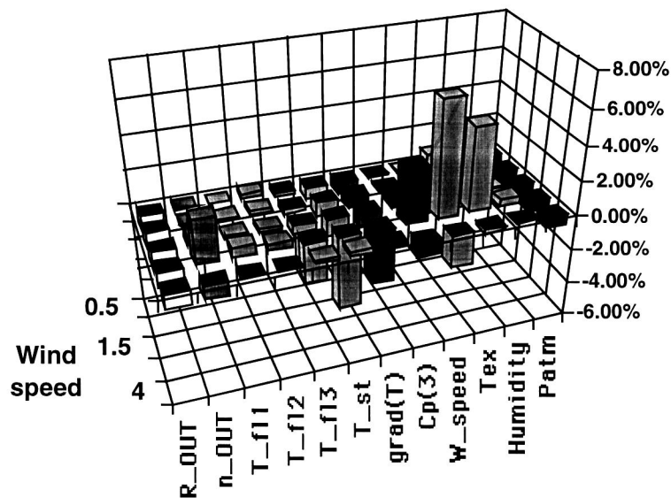
Figure 3: Evolution of the largest main effects with the wind speed
