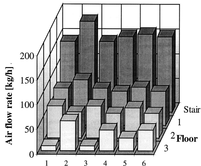
Figure 7: Comparison of mass air flow rates from Japanese user tests.
