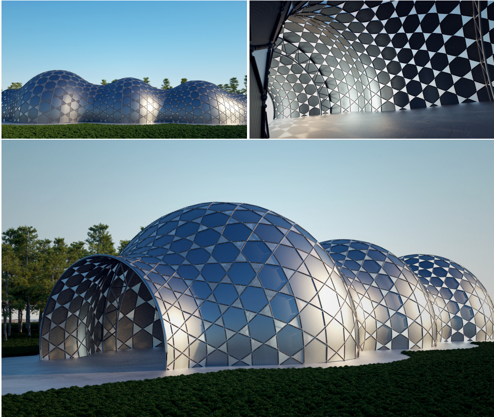
Figure 9: A hybrid shell structure integrates planar support arches in the interior into a deployable auxetic surface.
