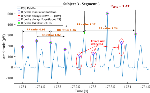
Fig. 11: ECG segment 5 (i.e., recovery after exhaustion) for Subject 3 with the R peaks from the three designs. For the misdetected small R peaks, the RR ratio is close to P_{99.5} but not enough to trigger an error.
