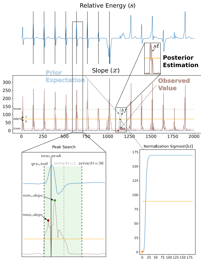
Fig. 6: Illustration of the main features of the BayeSlope algorithm. The bayesian filter (i.e., prior estimation), together with the generalized logistic function (normalization sigmoid) allows to locally enhance the observed slope value ( x ), leading to a posterior estimation that goes above the detection threshold. The bottom-left part of the figure illustrates the peak search procedure that is triggered once the detection threshold is surpassed. All symbol names correspond to those introduced in Algorithm 1.
