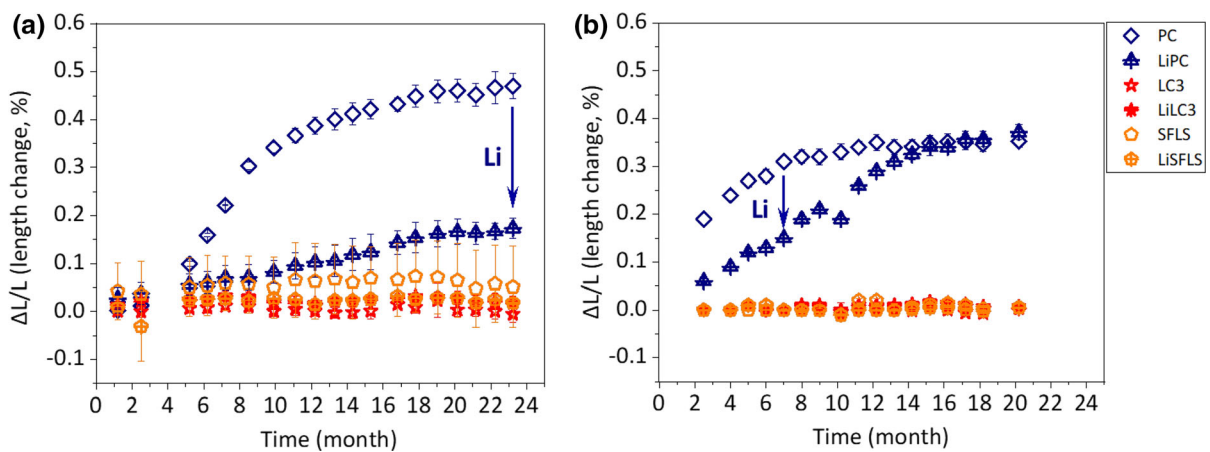
Fig. 5 The effect of Li addition (plus 400 mmol/L LiCl) on the extent of ASR-expansion for concrete prisms made of different pastes and U aggregate ( W/B = 0.46 ) as a function of time a at
