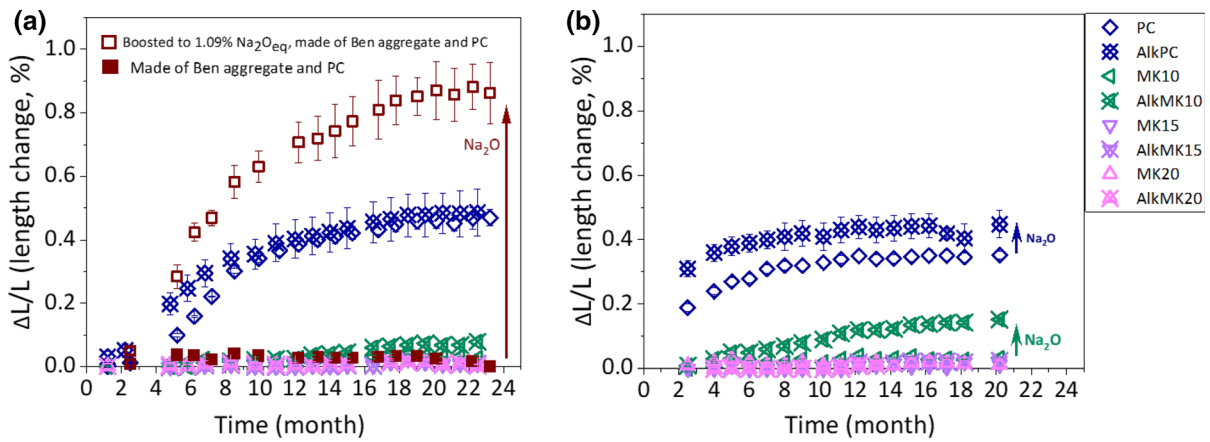
Fig. 4 The effect of extra alkali (boosted to 1.09% Na 2 O eq by adding NaOH) on the extent of ASR-expansion for concrete prisms made of different paste and U or Bend aggregate (filled
