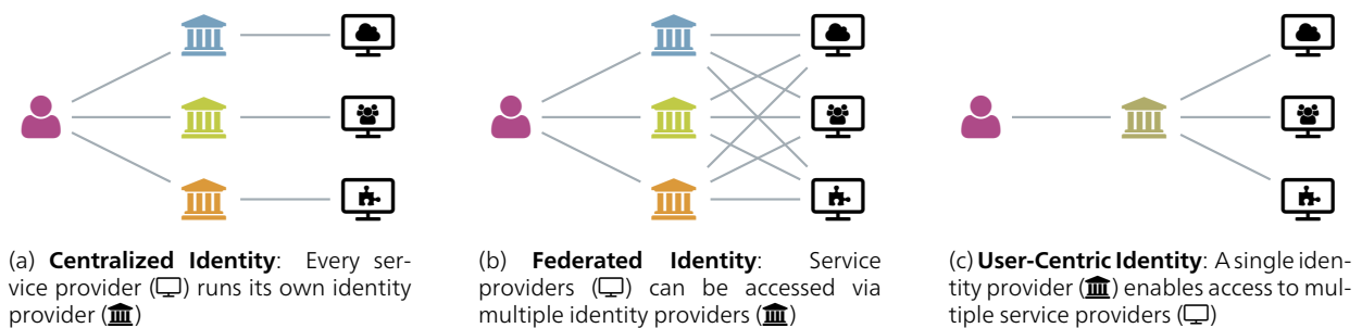
Figure 1.2: Different Models of Digital Identity (1/2)
