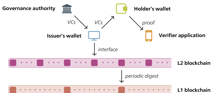
Figure 6.1: Components of SSI System
