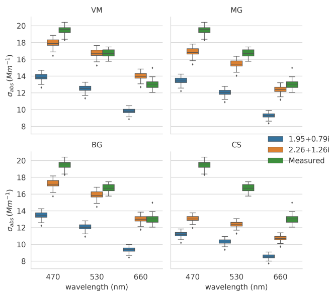
Figure 3. Modelled (blue and orange markers) and measured (green markers) absorption coefficients ( \sigma_{\text{abs}} ) at PSAP wavelengths for RF06_1. Variables are modelled with two m_{\text{BC}} values (shown in the legend) using the CS, MG, BG, and VM models (specified on the top of each plot). OA is assumed to be non-absorbing with the refractive index m_{\text{OA}} of 1.55 + 0i . The horizontal lines in the boxes represent the median value, the boxes represent the 25th to 75th percentile, the whiskers represent 1.5 times the interquartile range, and the diamonds represent outliers.
