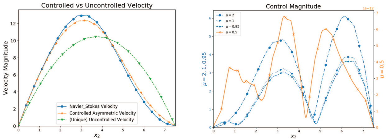
FIGURE 12. Distributed Control : Left : comparison of velocity profiles in the controlled and uncontrolled cases for \alpha = 0.01 , \mu = 2 . on \Gamma_{\text{obs}} w.r.t. the asymmetric desired profile when following the natural optimal branch. Right : representation of control variable evolution for \alpha = 0.01 , \mu = 2, 1, 0.95, 0.5 for x_1 = 45 when following the natural optimal branch.
