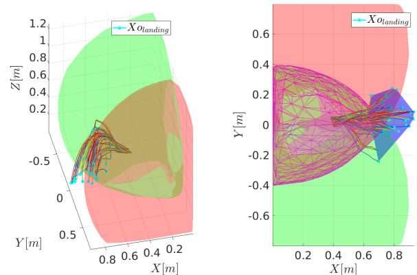
Figure 8. Extension of the dual-arm system's reachable space with the tossing reachable space. (left): set of 50 3D trajectories of tossed object with respect the dual-arm workspace (the green and red areas depict the left and right arms space of reachable positions). (right): top view of the tossing-based extension (blue area with the landing positions in cyan) of the joint reachable space depicted with the meshed region in magenta.
