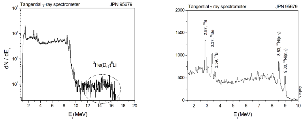
Figure 2. Gamma-ray spectrum recorded by the LaBr_3 detector in discharge #95679: (a) – a log-scale spectrum displays the detected 17-MeV gammas and (b) – a linear-scale zoomed spectrum clearly showing the gammas from the {}^9\text{Be}(D,n\gamma){}^{10}\text{B} and {}^9\text{Be}(D,p\gamma){}^{10}\text{Be} nuclear reactions.
