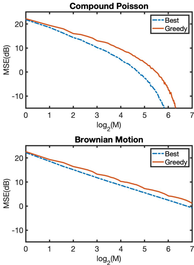
Fig. 3. Greedy and Best M -term approximation of a compound Poisson process (top) with \lambda = 10 and Gaussian jumps with a Brownian motion (bottom). We normalize both processes to have unit variance.
