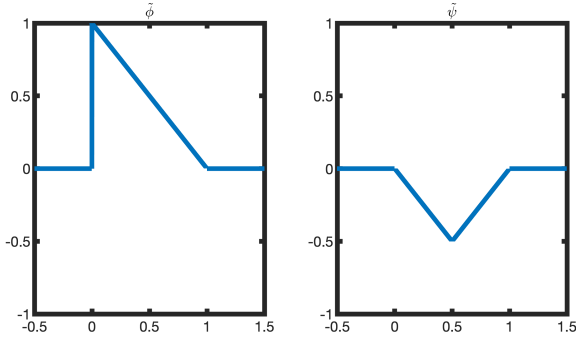
Fig. 5. Auxiliary functions \tilde{\phi} and \tilde{\psi}_{j,k} for j = 0, 1, 2 and k = 0, \dots, 2^j - 1 .
