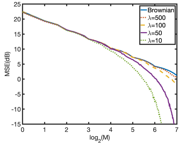
Fig. 2. Greedy approximations of Brownian motions and compound Poisson processes with different values of \lambda and Gaussian jumps. We fix the variance to one in all cases.
