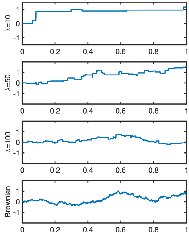
Fig. 1. Trajectories of compound Poisson processes with Gaussian jumps (different values of \lambda ) and a Brownian motion. All processes are normalized to have unit variance.
