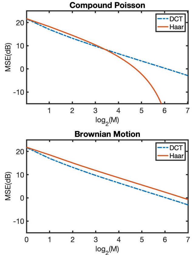
Fig. 4. Comparison of DCT versus Haar wavelets to optimally represent (best M -term) a compound Poisson process (top) with \lambda = 10 and Gaussian jumps with a Brownian motion (bottom). We normalize both random processes to have unit variance.
