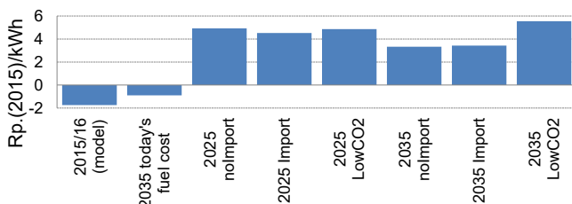
Figure 19: Scenario-dependent profitability of Swiss hydropower (average market revenues under assumption of 100% day-ahead trading).
