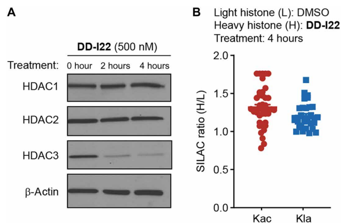
Fig. 7. Selective degradation of HDAC3 and mass spectrometric quantification of in vivo delactylation targets on core histones. (A) Changes in HDAC1–3 concentration upon treatment of HEK293 cells with PROTAC DD-I22 at 500 nM for the indicated time (see fig. S8 for chemical structure and optimization of degradation conditions in HeLa and HEK293T cells). (B) MS quantification of Kac and Kla sites on core histones extracted from HEK293 cells upon treatment with DD-I22 (500 nM) for 4 hours (see fig. S10 for quantification after 2 hours).
