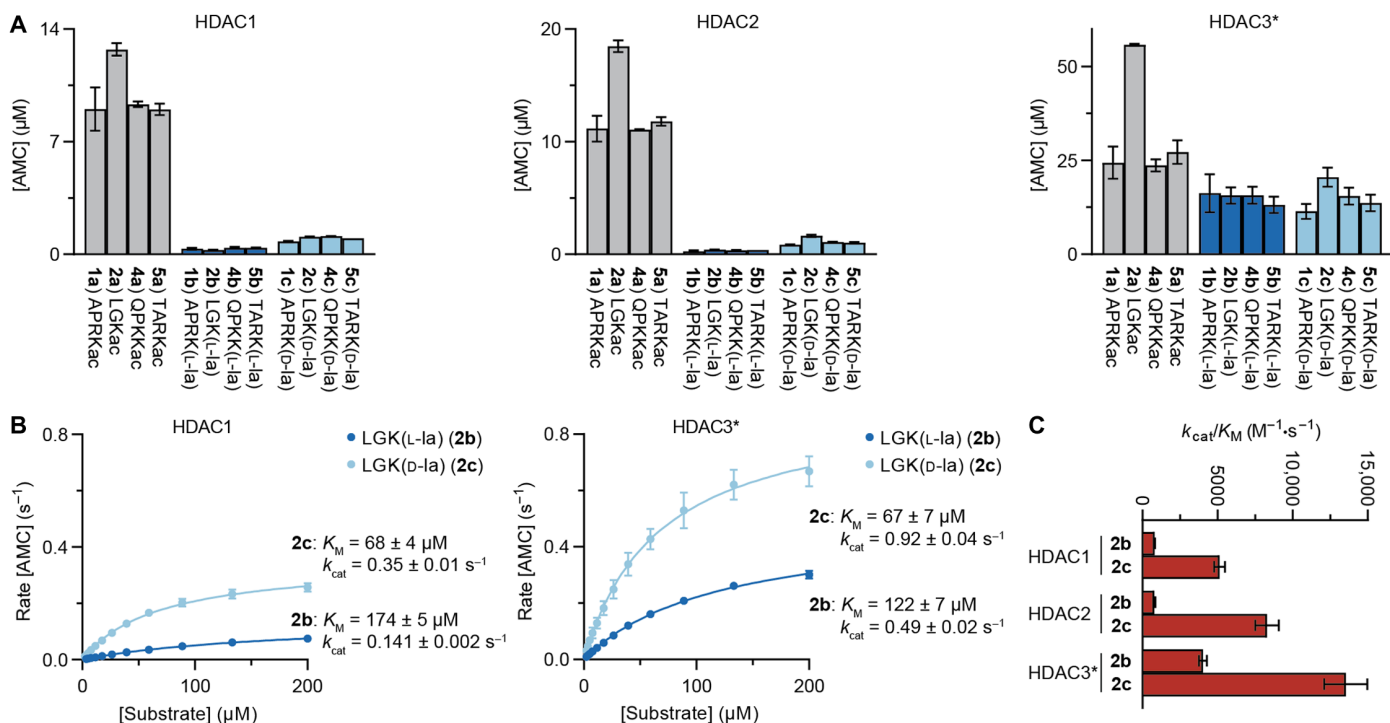
Fig. 2. Delactylase activity of class I HDAC1–3. (A) Conversion of Kac, K(L-la), and K(D-la) short AMC-conjugated peptides. Data represent means \pm SD ( n = 2 ). (B) Michaelis-Menten plots for HDACs 1 and 3 against substrates 2b and 2c . Data represent means \pm SEM ( n = 2 ) (see fig. S4 for HDAC2 data and sample assay progression curves). (C) Catalytic efficiencies of HDAC1–3 against substrates 2b and 2c . Data represent means \pm SEM ( n = 2 ) (see fig. S4 for complete K_M and k_{cat} datasets). *HDAC3 incubated with the DAD of NCoR2.
