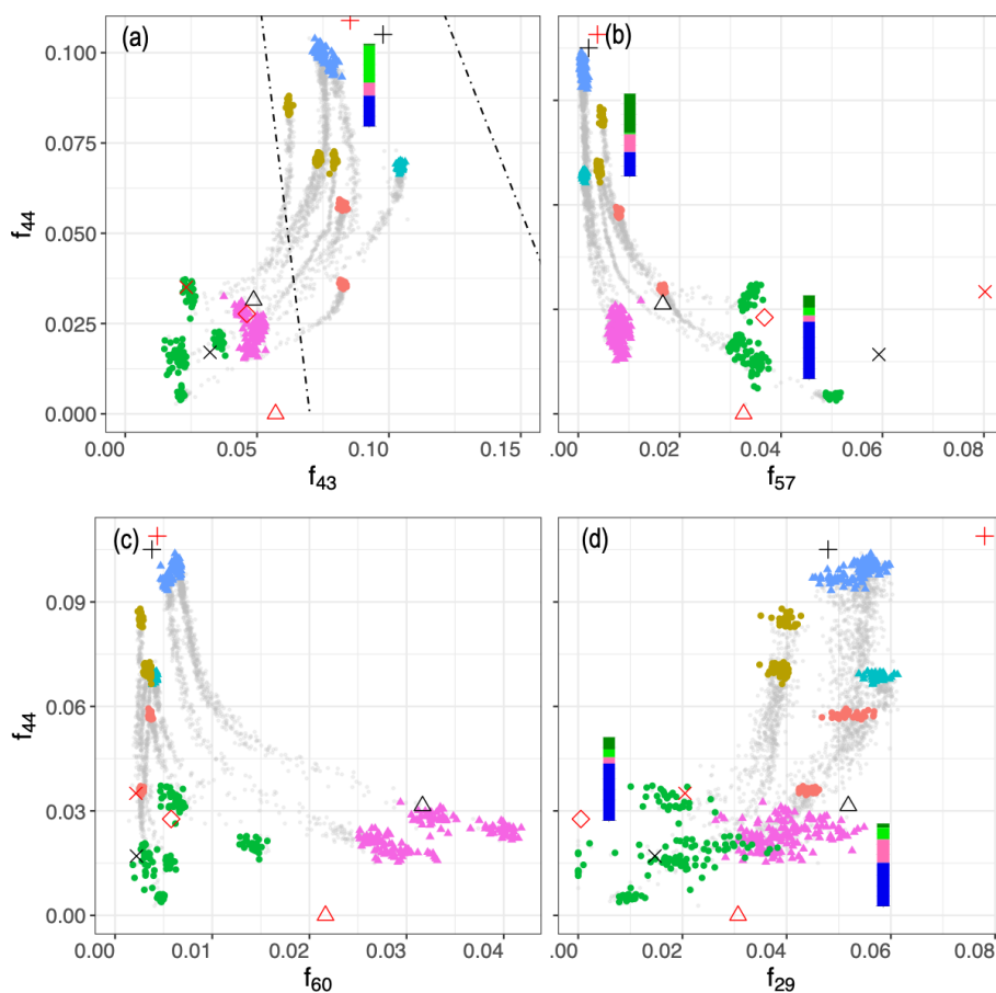
Figure 5. Scatter plots of f_{44} ( f_{\text{CO}_2^+} ) against f_{43} ( f_{\text{C}_2\text{H}_3\text{O}^+} ), f_{57} ( f_{\text{C}_4\text{H}_9^+} ), f_{60} ( f_{\text{C}_2\text{H}_4\text{O}_2^+} ), and f_{29} ( f_{\text{CHO}^+} ). Dashed lines show the outline of the triangle (Ng et al., 2010), and the black shapes show the location of PMF factors (Elser et al., 2016; Aiken et al., 2009; Ulbrich et al., 2009). Average FG composition for each category estimated from the MIR spectra are shown beside the category. Figure 4 legend is applicable here.
