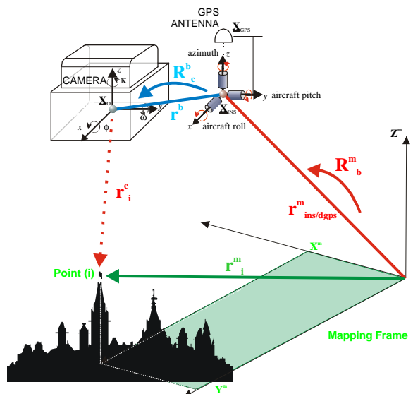
Figure 1. Elements of georeferencing by INS/DGPS.
