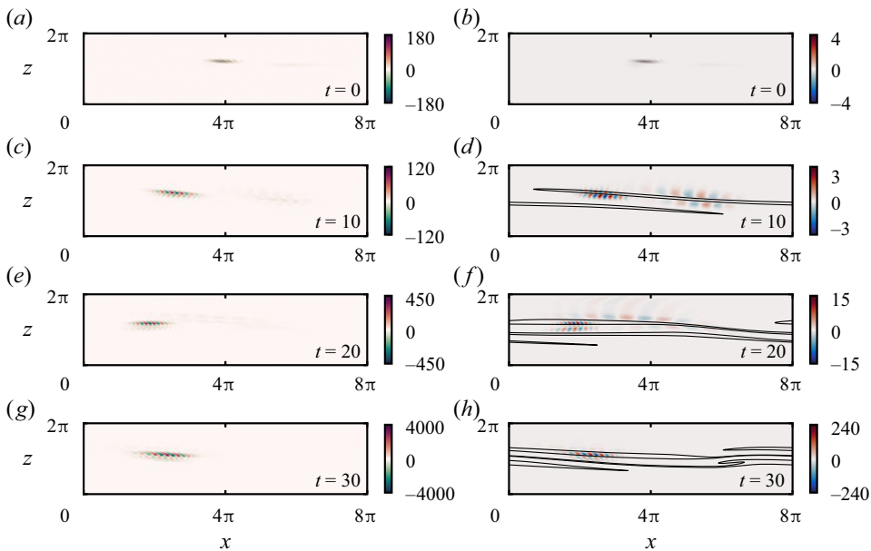
Figure 4. The x-z plane slices of the perturbation spanwise vorticity field \partial u'/\partial z - \partial w'/\partial x (a,c,e,g) and buoyancy b' (b,d,f,h) for the 2-D optimal perturbation (calculated using L_y = 0.1 ) with T = 30 . Alternating spanwise vortices are tilted and distorted by the background shear, as is typical of the Orr mechanism. The black contour on the right surrounds regions of negative (and hence statically unstable) background buoyancy gradient.
