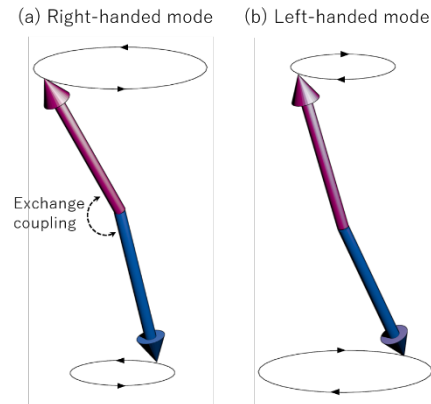
Figure 1 (a) the right-handed mode and (b) the left-handed mode of the antiferromagnetic dynamics
