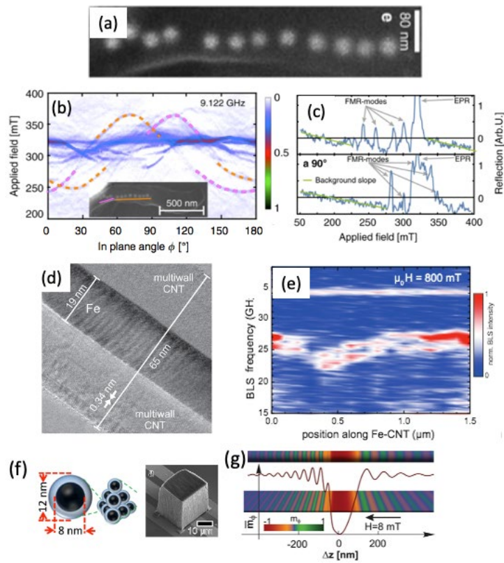
Figure 2: (a) Magnetite crystal chain grown by magnetotactic bacteria. (b) Angular dependence of magnetite crystal chain FMR spectra and (c) two single spectra recorded at 0^\circ and 90^\circ . (d) TEM of a single Fe filled carbon nanotube suspended across micro-resonator. (e) Thermal spin-wave spectrum of FeCNT obtained using BLS. (f) Schematic of \text{Fe}_3\text{O}_4 crystal monomer (left), crystals (middle) and an SEM of the machined \text{Fe}_3\text{O}_4 crystal upon a coplanar waveguide. (g) Spin-Cherenkov effect in magnetic nanotube.
