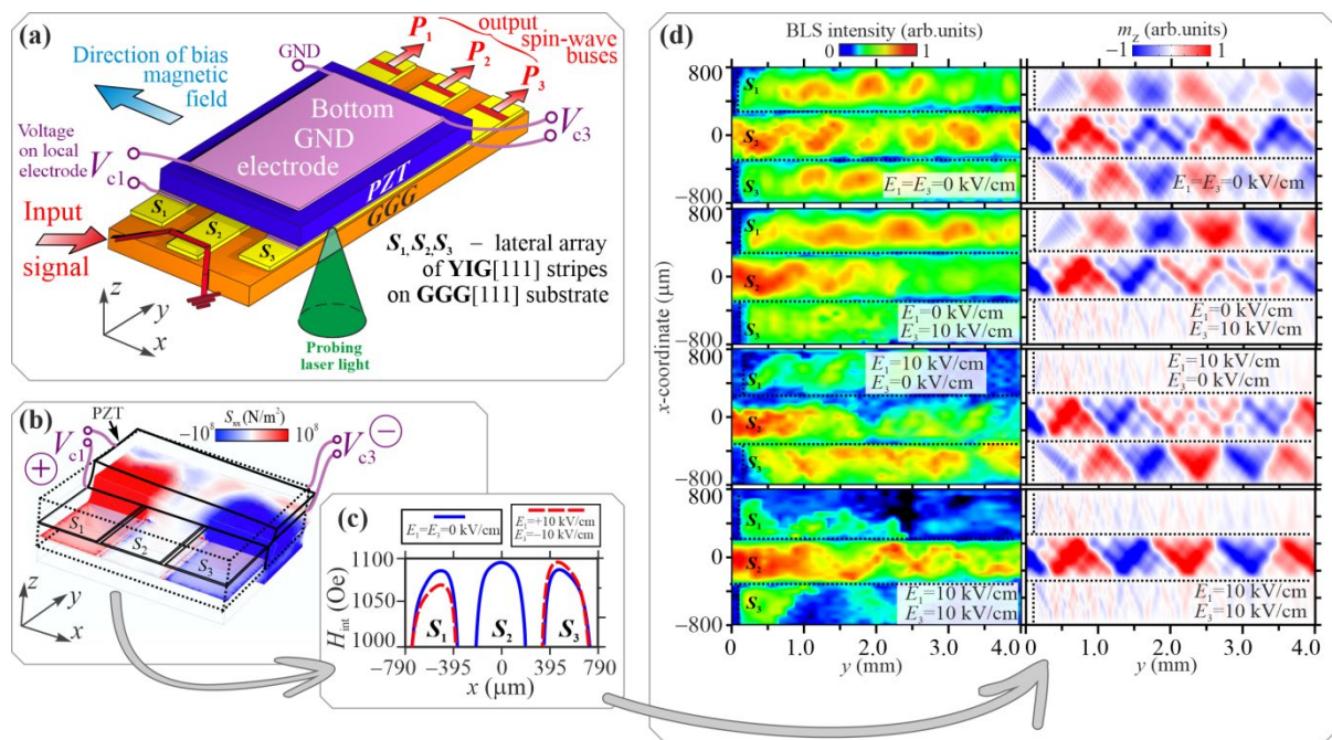
Figure 1. The demonstration of magnon straintronics concept: the bilateral YIG stripes ( S_1, S_2, S_3 ) with strain coupled PZT layer (a). The electric voltage is applied between two electrodes ( V_{c1} and V_{c3} ) at the YIG/PZT interface and GND electrode. The distribution of stress tensor component showing a local deformation of the PZT layer and induced stress on the YIG/PZT interface (b). The voltage-induced transformation of the internal magnetic field profile ( H_{int}(x) ) (c). Left panels of (d) show the BLS spin-wave intensity at the frequency of 4.925 GHz at the different values of the applied voltages (denoted in the figure). Right panels of (d) show snapshots of the dynamic out-of-plane component of dynamic magnetization calculated by means of micromagnetic simulations. Edges of stripes are guided with dotted lines. (From [2])
