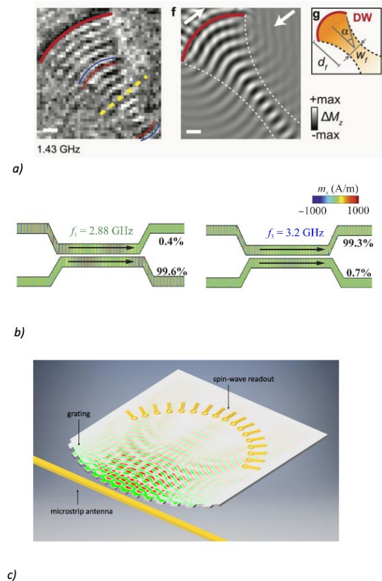
Figure 1. Examples of magnon-based optical processing (a) X-ray-based magnetic image of a spin wave lens, realized in a synthetic antiferromagnet [4], near-field coupled waveguides in YIG, with frequency-dependent coupling [6] and conceptual view of a Rowland-circle-based microwave spectrum analyser. Figures are used with permission.
