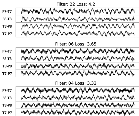
Fig. 10. Maximized inputs for kernels of the last convolutional block - 3x5 model. The three maximizing inputs eliciting the strongest activation after the last convolutional block of the 3x5 model are represented. This shows that the 3x5 model learned to make implicit representation of low frequency components of the EEG signal.
