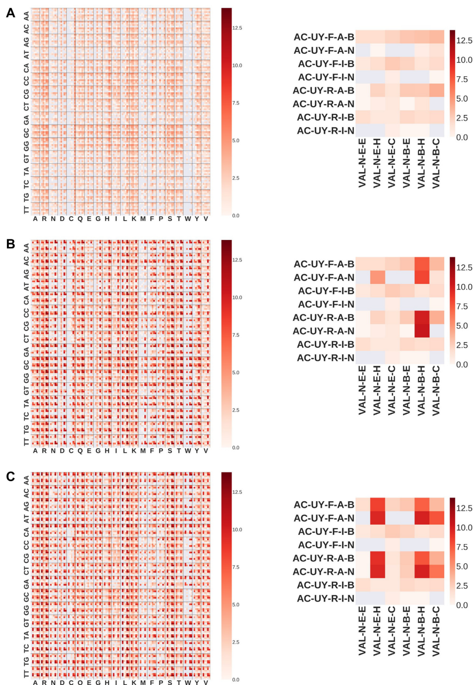
Figure 3. Heatmap plots of the number of amino acid—dinucleotides and their environments (etriads) at distance shorter than 30Å in a logarithmic scale. Detailed view of a cell of the heatmap is shown in the right side of each heatmap. Each square inside the cell shows the number of extended-triads (in logarithmic scale) for a specific amino acid—dinucleotide (the example uses valine, Val and adenosine-cytosine, AC) and their environments. Amino acid environments are: hydrophobicity (P as polar, N non polar), surface accessibility (E if exposed, B if buried) and secondary structure (E for \beta -strand, H for helix and C for coil). Dinucleotide environments are: type of nitrogenous bases (U for purine, I for pyrimidine), closest DNA strand (F for forward, R for reverse), closest DNA groove (A for major, I for minor) and closest chemical group (B if phospho-ribose backbone atoms, N if nucleobase). (A) Extended-triads obtained from PDB structures. (B) Extended-triads obtained from PDB structures and B1H experiments of the F2 domain. (C) Extended-triads obtained from PDB structures and B1H experiments of the F3 domain. A detailed analysis of panels A, B and C is available in the web repository ( http://sbi.upf.edu/C2H2ZF_repo ).
