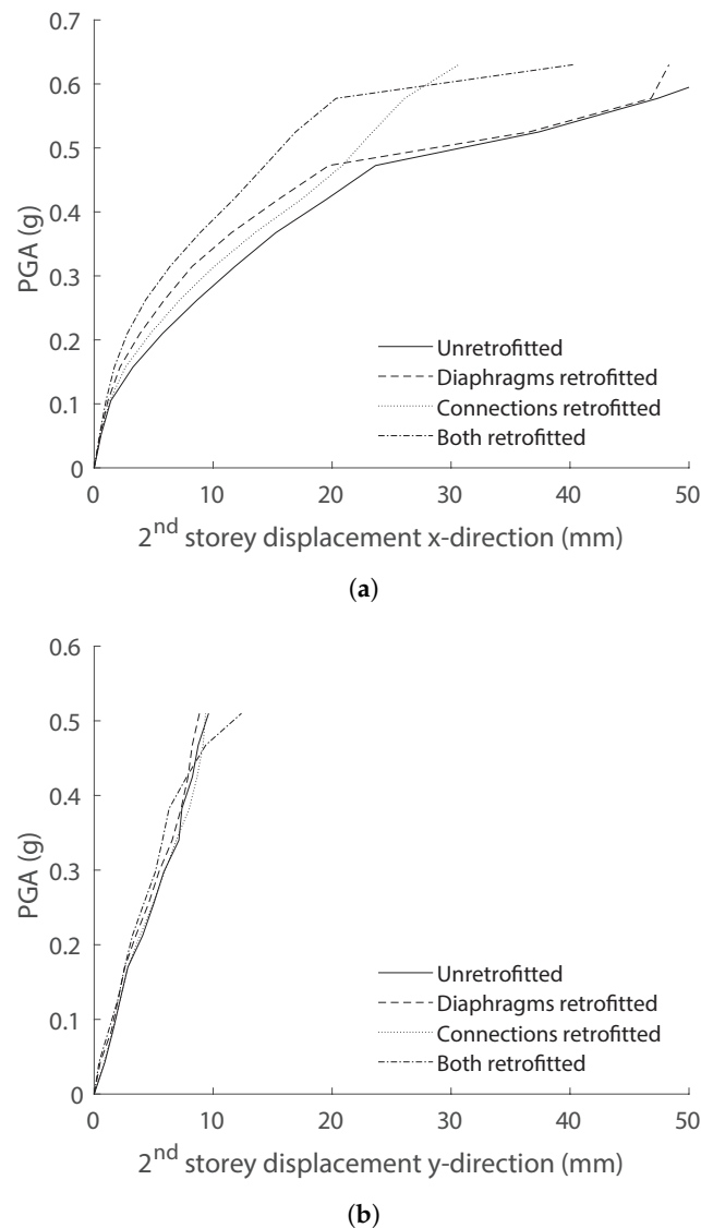
Figure 12. IDA curves for the four configurations in terms of PGA vs. the absolute maximum values of average 2nd storey displacement: (a) in the x-direction (b) in the y-direction.
