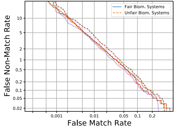
Fig. 4. DET curves for the canonical fair and unfair synthetic verification systems. It can be observed that analyzing this curves gives a false impression that the unfair synthetic verification system is fair.
