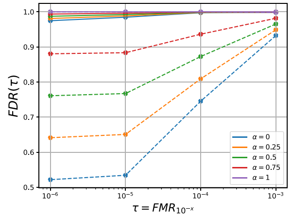
Fig. 6. FDR(\tau)|\alpha for different values of \alpha (see equation (6)). Solid lines represent the FDR(\tau)|\alpha for the synthetic fair verification system. Dashed lines represent the FDR(\tau)|\alpha for the synthetic unfair verification system.
