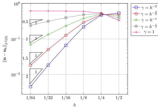
FIGURE 20. Compare L^2 -errors for the velocity in the “unit circle” using (20) with respect to different values of the penalty parameter \gamma with triangular elements.
