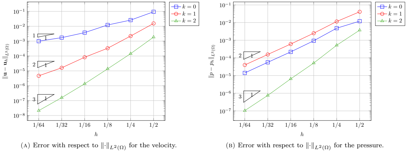
(A) Error with respect to \|\cdot\|_{L^2(\Omega)} for the velocity.
