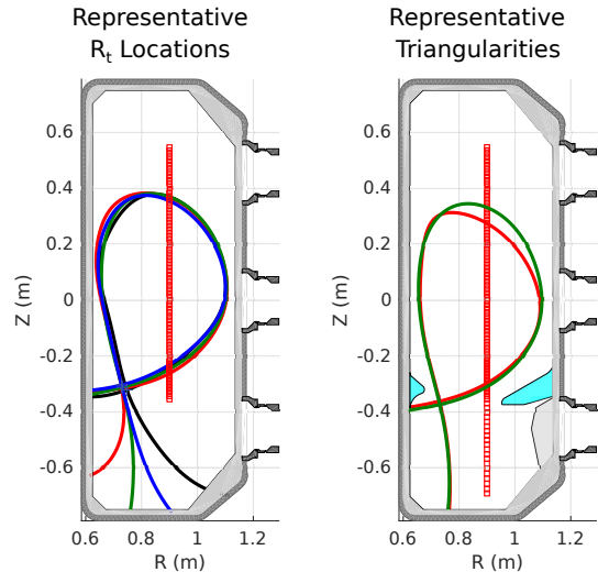
Figure 1: Left - Unbaffled TCV configuration with representative R_t locations. Thomson scattering measurement locations shown in red squares. Right - Baffled TCV configuration with two representative triangularities. Additional divertor Thomson scattering locations were installed with the baffles.
