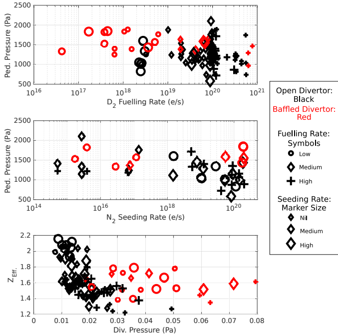
Figure 6: P_{ped} at varying fuelling (top) and nitrogen seeding (middle) rates. Z_{eff} as a function of divertor pressure (bottom).
