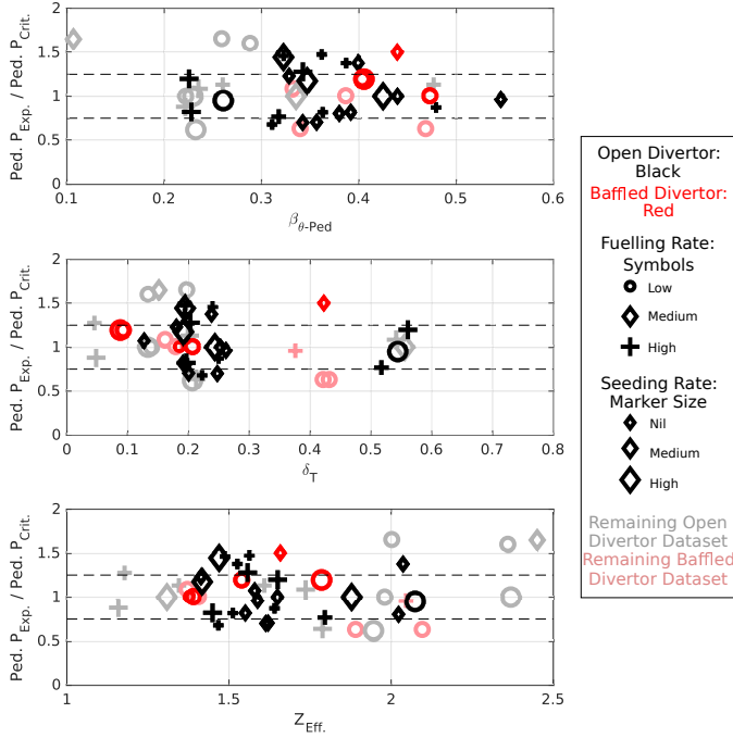
Figure 8: Ratio of experimental pedestal pressure and critical pedestal pressure with pedestal \beta_\theta (top), \delta_T (middle) and Z_{\text{eff}} (bottom). Faded symbols indicate the database not selected in experimental analysis. The dashed lines indicate a ratio of \pm 0.25 .
