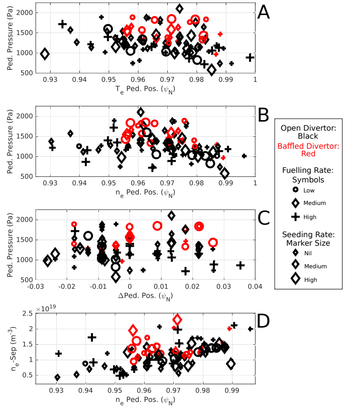
Figure 7: Pedestal top pressure variation with T_e pedestal position (A), n_e pedestal position (B) and difference in T_e and n_e pedestal positions (C). n_e - Sep as a function of n_e pedestal position (D).
