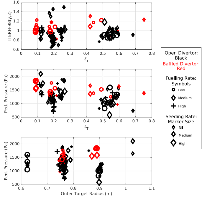
Figure 5: ITERH-90(y,2) (top) and P_{ped} (middle) with \delta_T . P_{ped} as a function of R_t (bottom).
