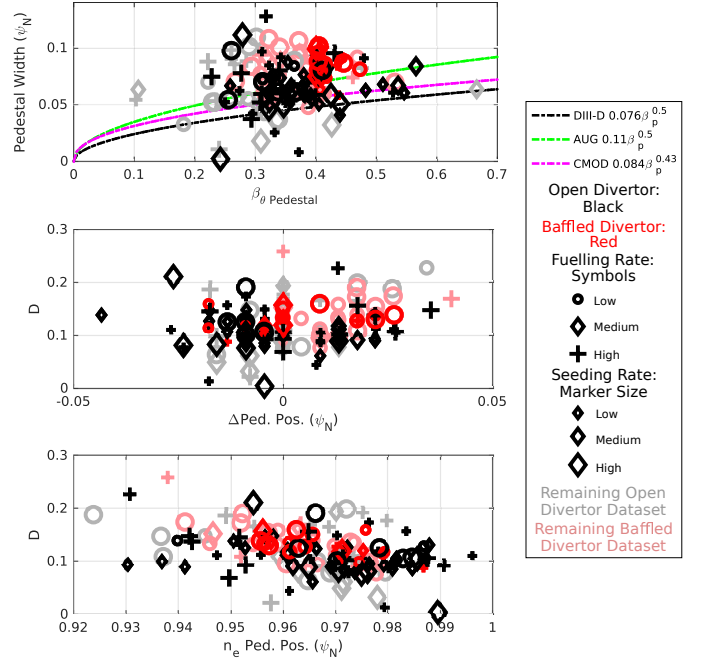
Figure 9: Pedestal width as function of \beta_\theta^{\text{Ped.}} (top). Relations observed on DIII-D, AUG and CMOD indicated with dashed lines. D with relative pedestal position (middle) and n_e pedestal position (bottom). Faded symbols indicate the remaining database not selected in the detailed analysis.
