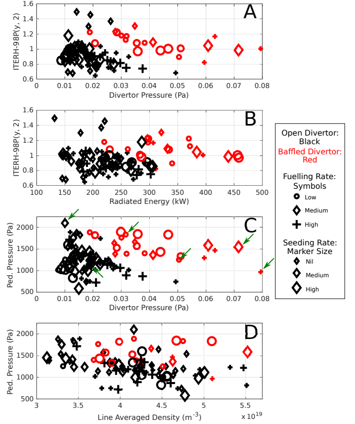
Figure 3: ITERH-98(y,2) as function of divertor pressure (A) and ELM averaged total radiated energy (B), P_{ped} as a function of divertor pressure (C) and line averaged density (D). Green arrows in (C) indicate discharges with the same NBH power coupled to the plasma.
