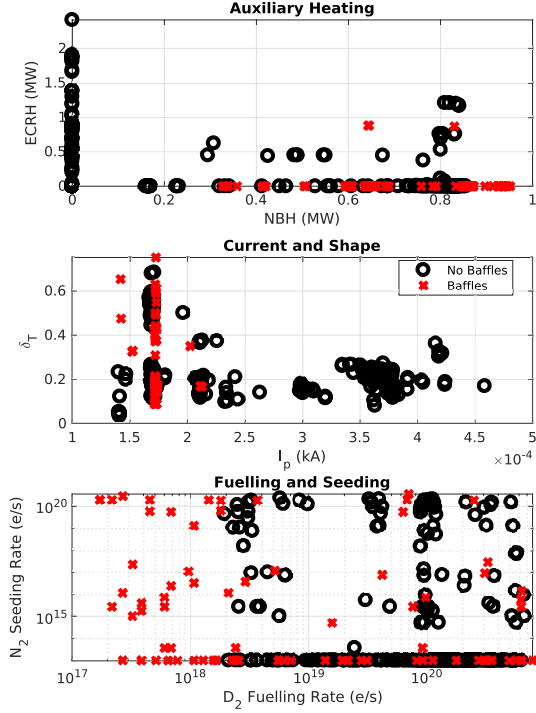
Figure 2: Overview of discharges analysed. Top - Injected auxiliary heating power, middle - upper triangularity and plasma current, bottom - nitrogen seeding and fuelling rates.
