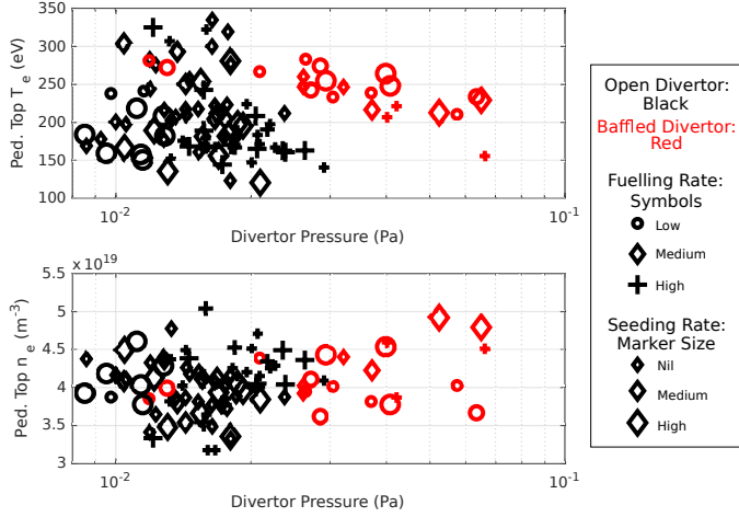
Figure 4: Pedestal top T_e (top) and n_e (bottom) with divertor neutral pressure.
