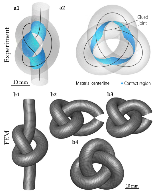
Fig. 2. Methods to realize and analyze the elastic open and closed trefoil knots. a1 , Rendering of the reconstructed \mu CT-data of an experimental open trefoil knot with a normalized knot length \Lambda_{oc} = 85.9/D_0 = 10.1 . a2 , Rendering of the reconstructed \mu CT-data of the elastic closed trefoil knot with a length-to-diameter ratio of L_0/D_0 = 16.37 . b1 , FEM computed equilibrium shape of an open trefoil knot. b2-b4 , Successive rod-end displacements to obtain the FEM closed configuration starting from a tight open trefoil knot.
