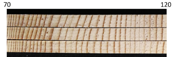
Fig. 20. Mesostructure of specimens TT-120-14-REB5 (top), TT-120-15-REB5 (middle) and TT-120-16-REB5 (bottom). Dimensions are in mm.
