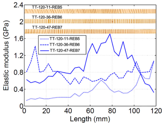
Fig. 16. Correspondence between mesostructure of spruce and local transverse elastic modulus.
