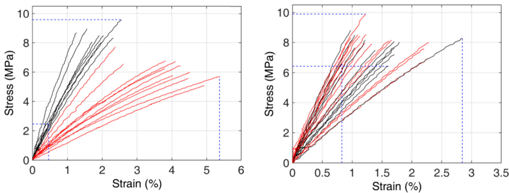
Fig. 7. Transverse tensile stress–strain curves of spruce wood for 32-mm specimens cut from REB3 (left) and REB4 (right).
