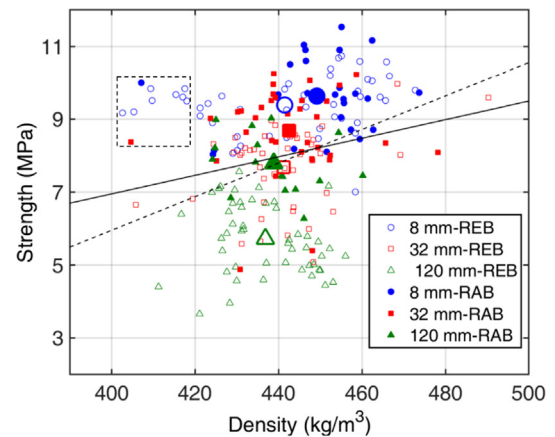
Fig. 15. Correlation between density and tensile transverse strength. Solid line – regression line for all data, dashed line – regression excluding the outliers (data in the box).
