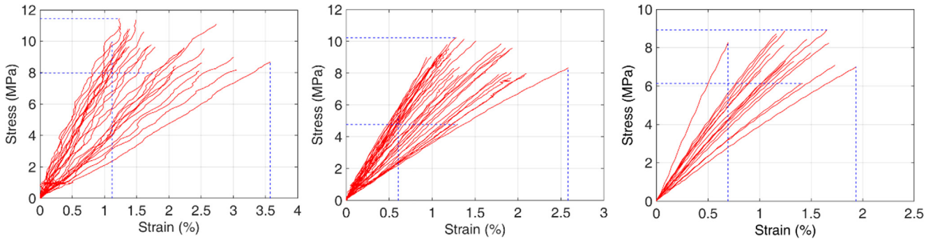
Fig. 11. Transverse tensile stress–strain curves of spruce wood for 8-mm specimens (left), 32-mm specimens (middle) and 120-mm specimens (right), cut from RABs.
