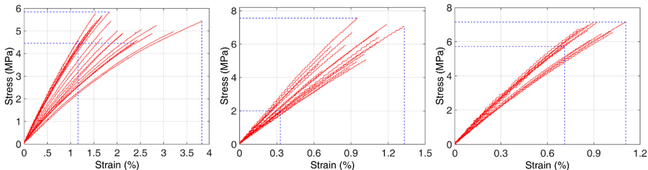
Fig. 8. Transverse tensile stress–strain curves of spruce wood for 120-mm specimens cut from REB5-REB7 (left–right).
