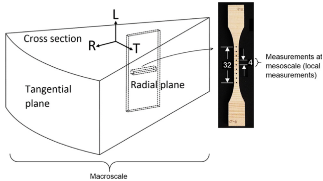
Fig. 1. Schematic illustration showing the principal directions, planes, and approximate position of boards (not in scale). Dimensions in mm.
