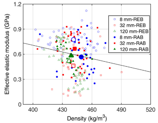
Fig. 14. Correlation between density and effective elastic modulus.
