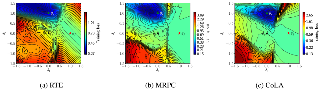
Figure 7: 2D loss surfaces in the subspace spanned by \delta_1 = \theta_f - \theta_p and \delta_2 = \theta_s - \theta_p on RTE, MRPC, and CoLA. \theta_p, \theta_f, \theta_s denote the parameters of the pre-trained, failed, and successfully trained model, respectively.
