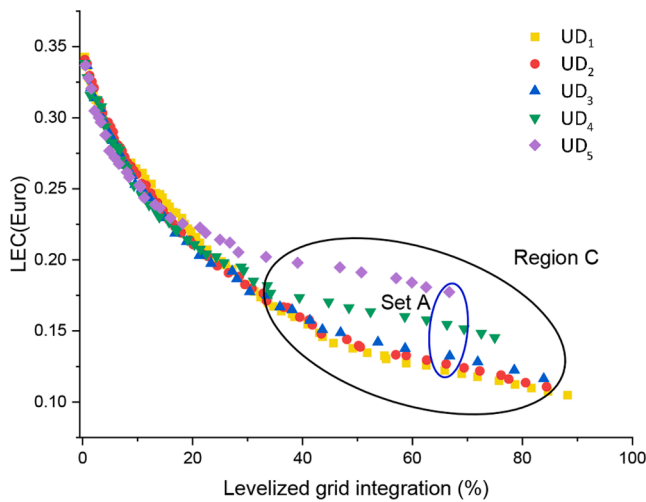
Fig. 12. Variation of Levelized Energy Cost (LEC) along with leveled grid integration level for the Pareto solutions.
