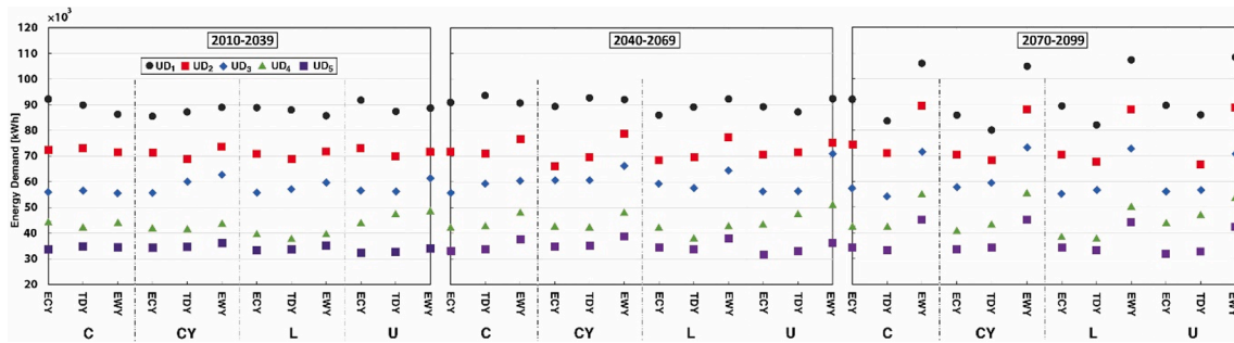
Fig. 9. Peak energy demand for all urban morphologies based on UDs and forms for ECY, TDY, and EYW (2010–2039, 2040–2069, and 2070–2099).
