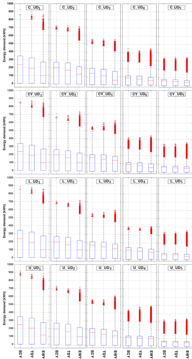
Fig. 6. Boxplot of annual energy demand for all urban morphologies based on UDs and forms (2010–2039).
