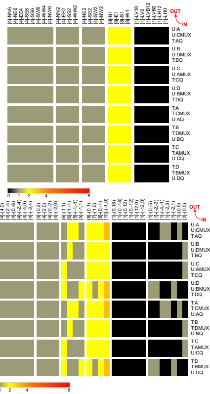
Figure 17: Adjacency of CLB outputs and wires. Top, clustering by name; bottom, direction-vector clustering.
