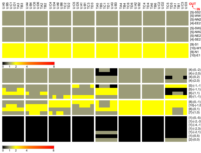
Figure 16: Adjacency of wires and LUT inputs. Top, clustering by name; bottom, direction-vector clustering. Wires longer than LEN-2 are omitted for they do not connect to CLB inputs.
