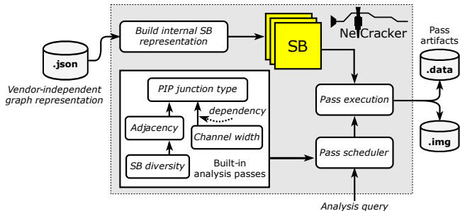
Figure 4: NetCracker architecture.
