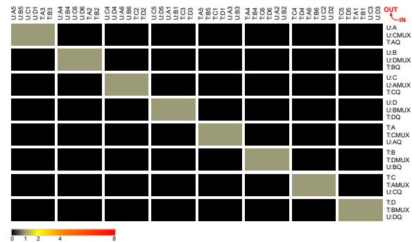
Figure 18: Adjacency of CLB outputs and LUT inputs.
