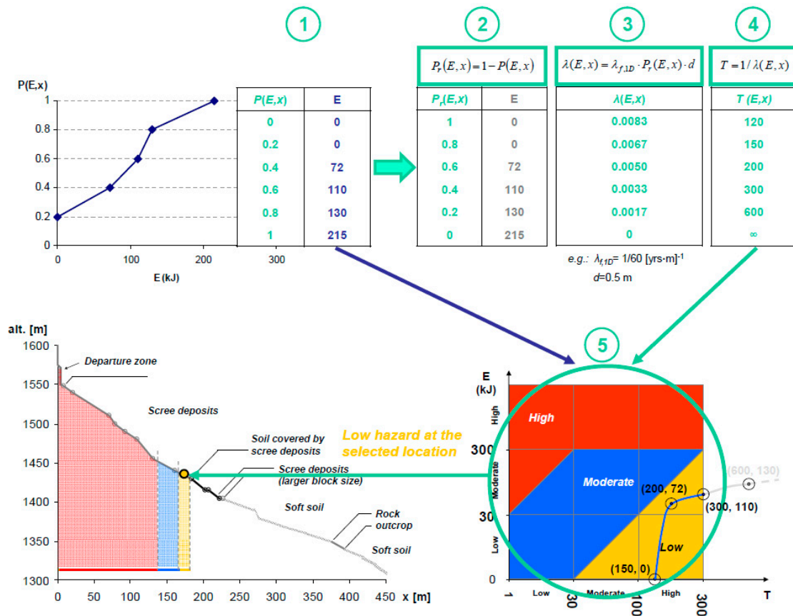
Figure 1. Steps of the new Cadanav methodology for one-dimensional zoning, after a failure frequency per unit length has been defined and trajectory simulations run. (1) Cumulative energy-probability distribution E-P(E, x) determined from raw trajectory modelling results—an initial value of 0.2 means that 20% of the blocks stopped before the selected location; (2) computation of probability of reach P_r(E, x) , (3) frequency of occurrence \lambda(E, x) and (4) return period T(E, x) corresponding to each energy value E ; (5) superimposition of the E-T couples to an intensity frequency diagram for hazard qualification.
