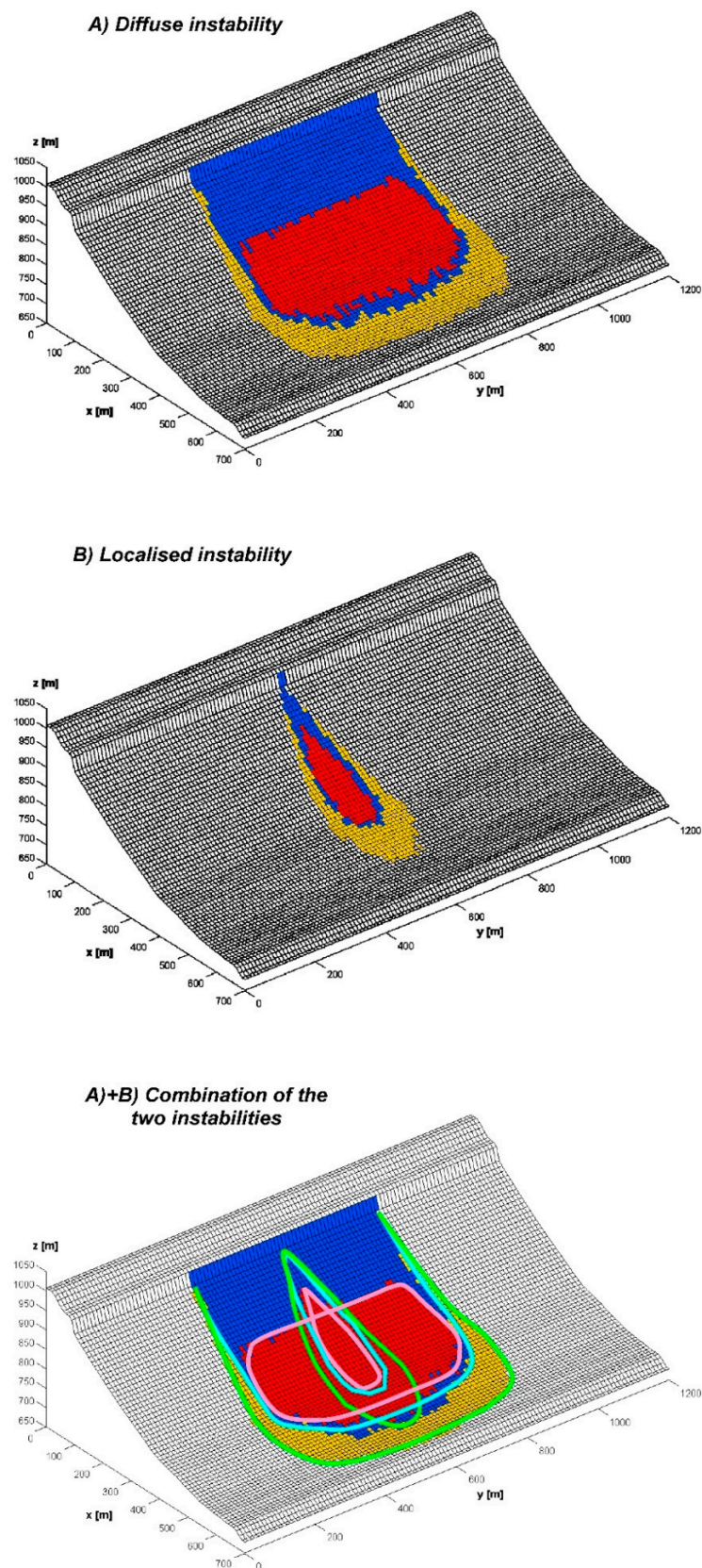
Figure 10. Combination of a diffuse ( \lambda_{f,2D} = 0.002 ( \text{years}^{-1} \cdot \text{m}^{-2} ), i.e., \lambda_{f,cell} = 0.2 \text{years}^{-1} ) and a localised instability ( \lambda_{f,2D} = 0.02 ( \text{years}^{-1} \cdot \text{m}^{-2} ), i.e., \lambda_{f,cell} = 2 \text{years}^{-1} ) for a linear cliff slope geometry. The boundaries of each of the two separate hazard zoning maps (A) and (B) are superimposed to the map obtained from their combination, (A) + (B).
