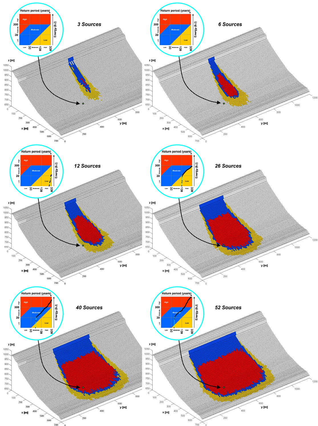
Figure 8. Hazard zoning for increasing number of rock fall sources along a linear cliff, for a failure frequency of \lambda_{f,2D} = 0.0038 (years -1 ·m -2 ) (i.e., \lambda_{f,cell} = 0.38 years -1 ). The hazard curve superimposed to the intensity-frequency diagram helps in understanding how a point located relatively far from the source area can be affected by a hazard whose degree increases according to the combined effect of an increasing number of sources of instability.
