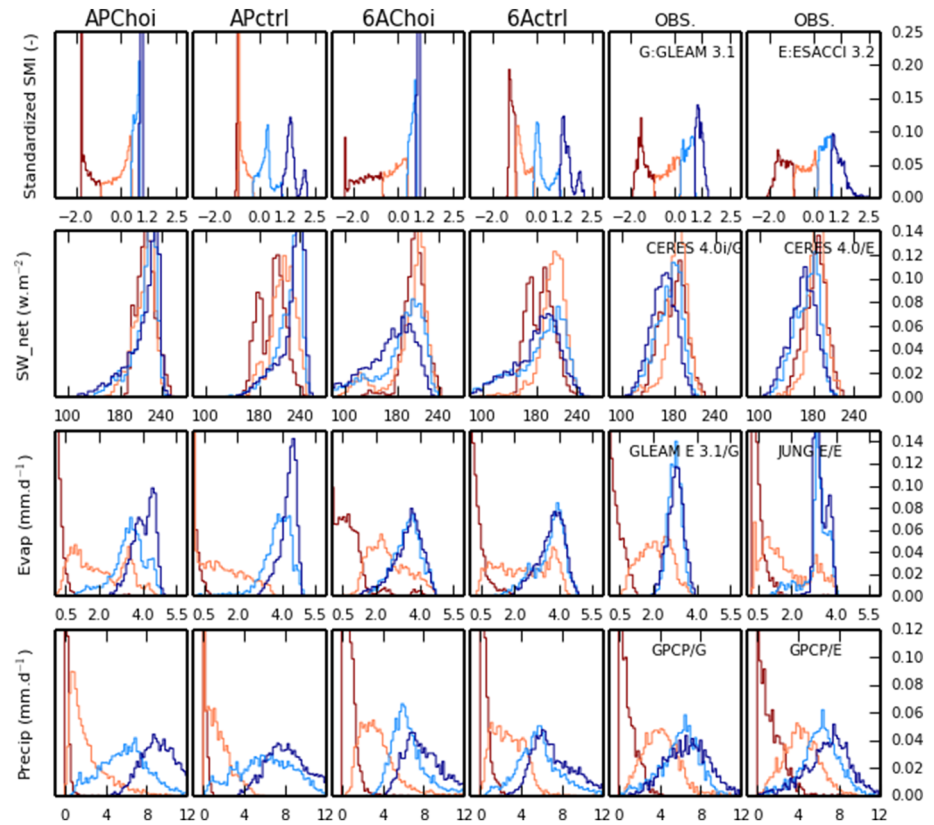
Figure 11. Regional histograms computed from monthly values of the individual grid points corresponding to the Sahel box ( -10:30^{\circ}\text{E} , 0:20^{\circ}\text{N} ) in JJA. The histograms are constructed for a 10-year long period in which all observations are available (2001–2010). Each row is dedicated to a particular variable: surface standardized soil moisture (first row), net SW radiation at the surface (second row), evaporation (third row), and precipitation (fourth row). The first four columns correspond to the reference experiments, and the last two columns correspond to the different sets of observations indicated above the corresponding histograms. The colors depict the PDF from the minimum to first quartile (dark red) from first quartile to the median (pale orange), from median to third quartile (cyan line), and from the third quartile to the maximum (blue line). For soil moisture, the y-axis is cut at .25 (representing 25% of the quartile) for the sake of readability but the driest quartile peaks at 0.8 (corresponding to 80% of the quartile) for APctrl and the moister quartile peaks at .8 for APchoi and APctrl. For evaporation they-axis is cut at .14 (corresponding to 14% of a quartile), but 55% (APchoi) and 90% (APctrl) of the evaporation associated with the first quartile is less than 0.1 mm/day. For the precipitation, the y-axis is cut at .12, but 70%, 85%, 15%, and 40% of the precipitation associated with the driest soil moisture quartile are less than 0.1 mm/day for APchoi, APctrl, 6Achoi, and 6Actrl and 20% and 10% for GLEAM and ESA-CCI.
