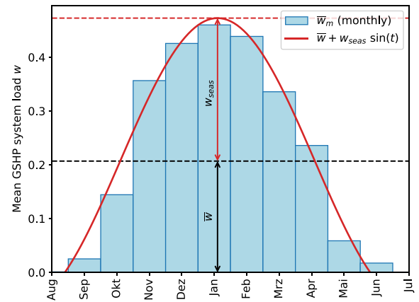
Fig. 3. Example of the monthly mean GSHP system load ( \bar{w}_m , blue bars, as fraction of the full load) and its sinusoidal approximation ( \bar{w} + w_{seas} \sin(t) , red line), based on the HDD of a representative location for western Switzerland (weather station of Pully) with a heating season of \sim 6 months. (For interpretation of the references to colour in this figure legend, the reader is referred to the Web version of this article.)
