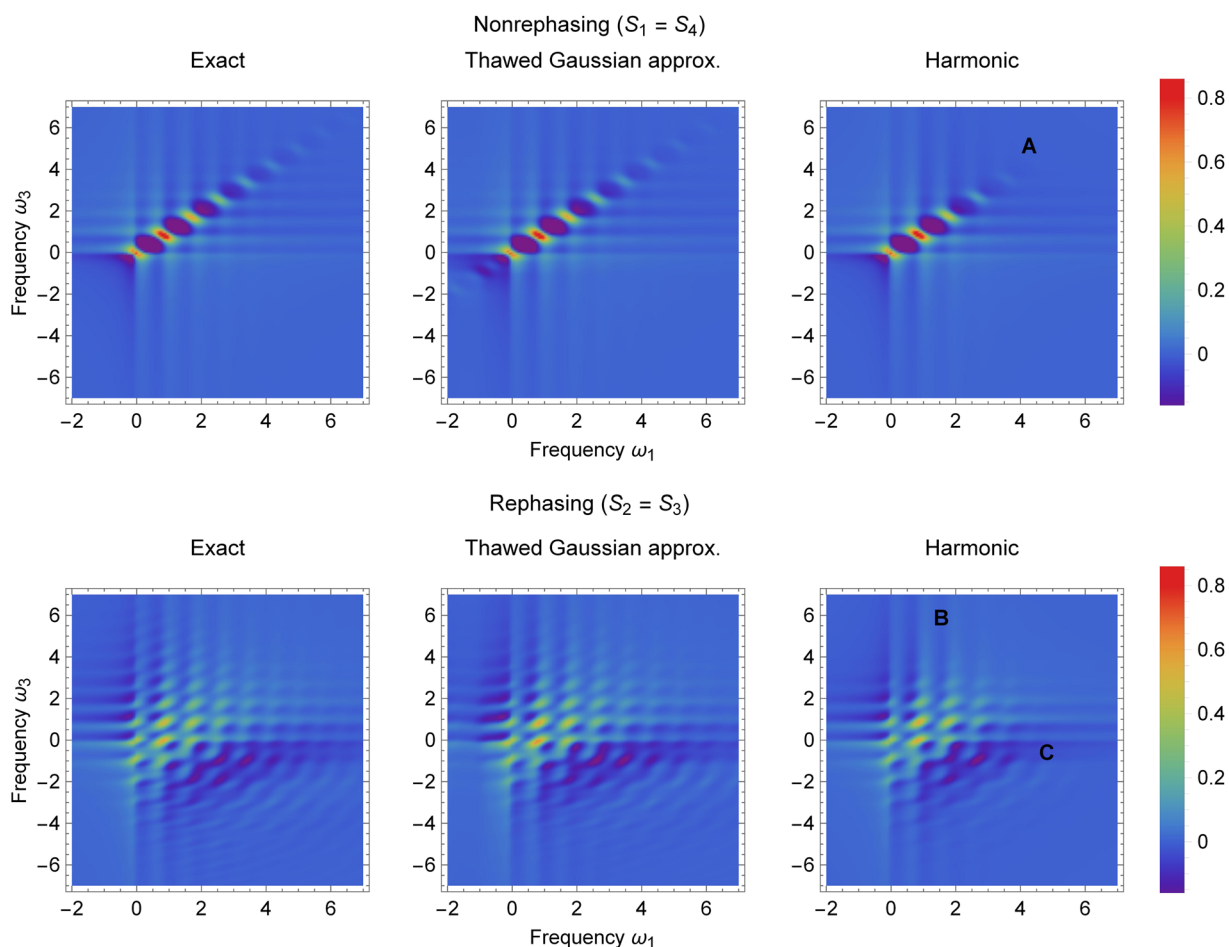
FIG. 2. Exact, thawed Gaussian, and harmonic two-dimensional electronic spectra of the harmonic-Morse system described in Sec. III A with the anharmonicity of the excited-state Morse potential \chi = 0.01 . Spectral regions A, B, and C, discussed in the main text, are indicated on the harmonic spectra.
