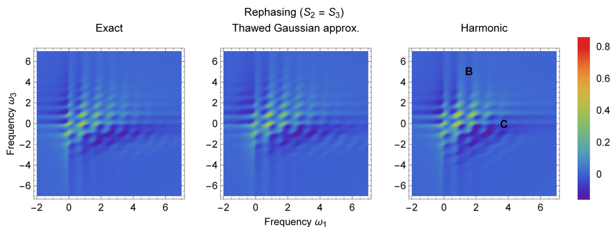
FIG. 4. Exact, thawed Gaussian, and harmonic rephasing spectra of the Morse–Morse system described in Sec. III A (anharmonicity \chi = 0.01 ).
