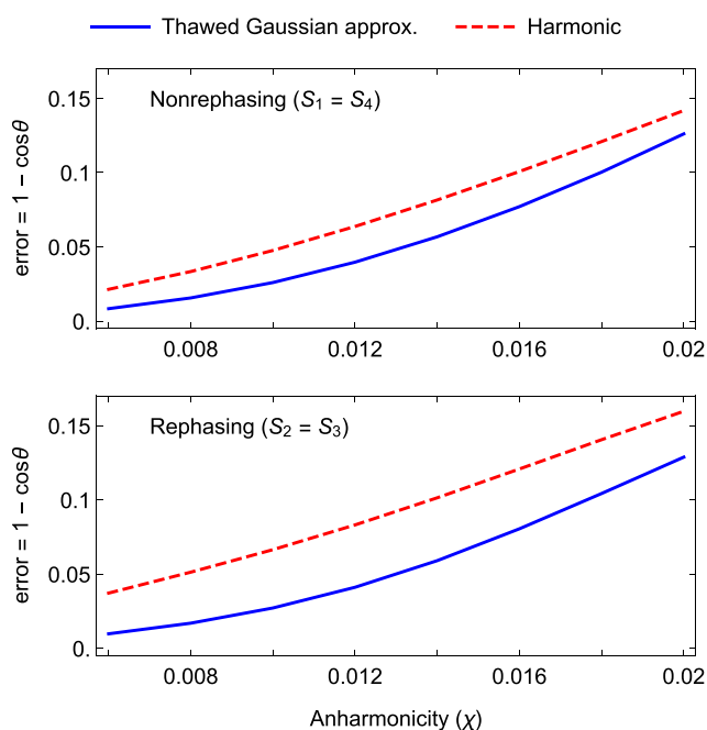
FIG. 3. Errors of the thawed Gaussian and harmonic spectra of the harmonic-Morse system, measured by the spectral contrast angles [Eq. (20)] at different values of the anharmonicity parameter \chi .
