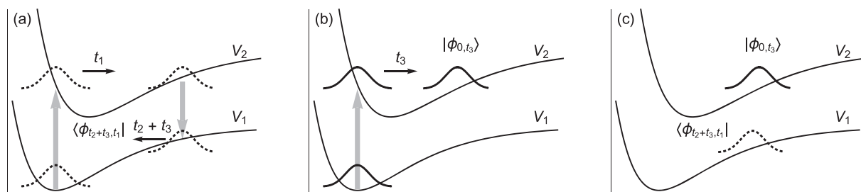
FIG. 1. Evolution of the bra [(a), dotted line] and ket [(b), solid line] wavepackets of Eqs. (7) and (11) for \tau_a = t_1 , \tau_b = t_2 + t_3 , and \tau_c = t_3 . Their overlap (c) is the R_3(t_3, t_2, t_1) component of the third-order response function R(t_3, t_2, t_1) [see Eqs. (5), (7), and (11)].
