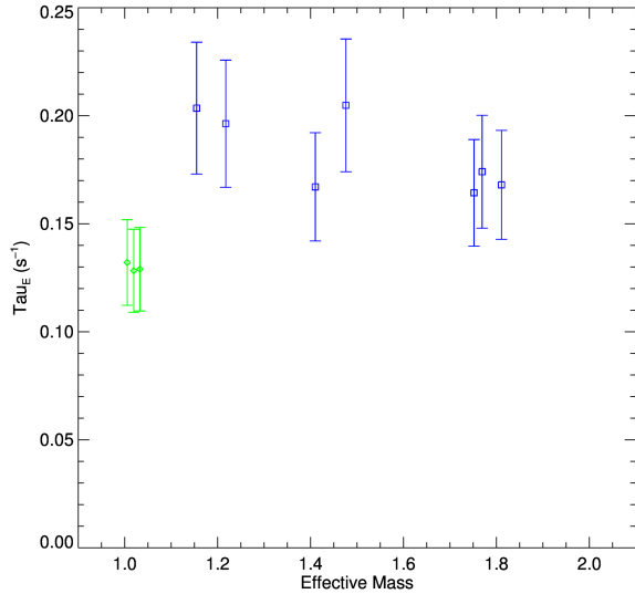
Figure 6: Thermal energy confinement time calculated by TRANSP vs effective mass for mixed isotope plasmas (blue) including plasmas with very low deuterium content (green)
