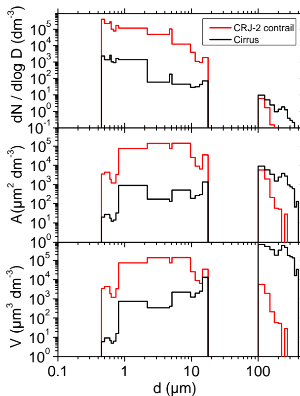
Fig. 10. Particle size, surface and volume distributions of the CRJ-2 contrail (red) embedded in a cirrus cloud (black). The ice surface area (ice volume) is given in \mu\text{m}^2 \text{ dm}^{-3} air ( \mu\text{m}^3 \text{ dm}^{-3} air) for each size bin. The total ice surface area and total ice volume can be calculated by summing up the individual size bins.
