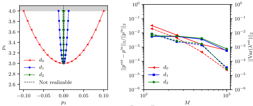
Fig. 7. Left: Input points depicted in (p_3, p_4) plane with black dashed line depicting p_3 = 0 with p_4 > 3 , Right: Average of moments relative error using data-driven MED for input moments p^{in} \in S_p^{test} , and variance of the predicted Lagrange multipliers shown in solid and dashed lines, respectively.
