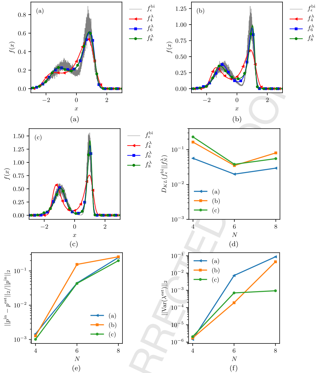
Fig. 10. Estimating the noisy bi-modal distribution f_\epsilon^{\text{bi}} with GP-accelerated MED f_N^\lambda , where N \in \{4, 6, 8\} for test cases \{(a), (b), (c)\} . Probability density functions are shown in (a)-(c). Also the KL-divergence between distributions, the relative error in outcome moments and the variance of the Lagrange multipliers are shown in (d)-(f), respectively.
