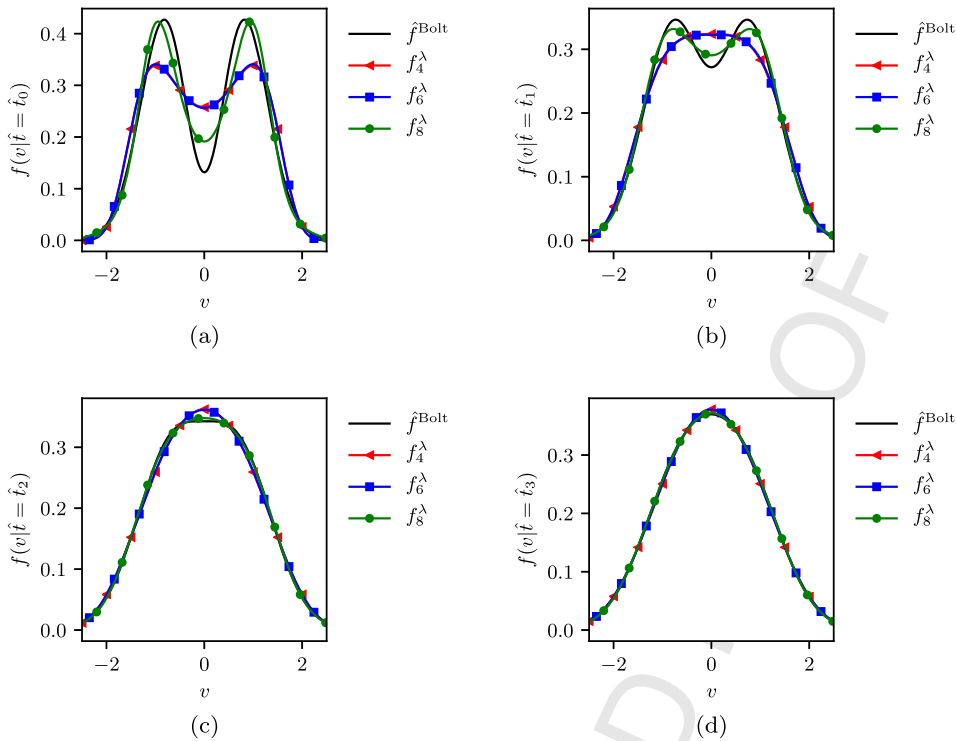
Fig. 13. Estimating solution of the Boltzmann equation at time \hat{t} \in \{5.8, 6.5, 7.5, 8.5\} by devised GP-accelerate MED for N = 4, 6 and 8 moments.
