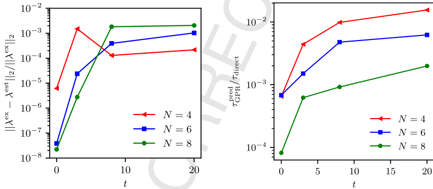
Fig. 12. Left: Relative error of the GP regression in predicting Lagrange multipliers of MED for N = 4, 6 and 8 , Right: The ratio between computational times required by direct and GP approaches for N = 4, 6 and 8 at time t \in \{0, 3, 8, 20\} .
