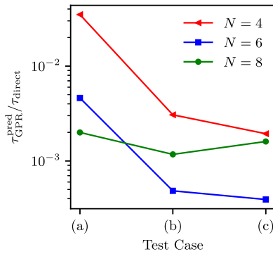
Fig. 9. The ratio between computational times of the GP regression and the direct approach are shown for computing the Lagrange multipliers.
