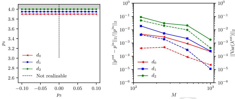
Fig. 6. Left: Input points depicted in (p_3, p_4) plane with black dashed line depicting p_3 = 0 with p_4 > 3 , Right: Average of moments relative error using data-driven MED for input moments p^{in} \in U_p^{test} , and variance of the predicted Lagrange multipliers shown in solid and dashed lines, respectively.
