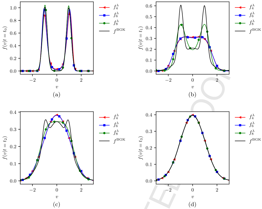
Fig. 11. Capturing BGK relaxation using GP-accelerated MED for N = 4, 6 and 8 moments at time t \in \{0, 3, 8, 20\} .
