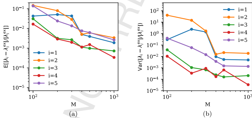
Fig. 2. Expectation and variance of the relative error in predicting \lambda_s using RBF. Here, \lambda^{\text{ex}} \in \mathbb{R}^N with N = 6 indicates the exact solution of MED taken from untrained subset of the data set. The statistics are performed over 2000 testing points.
