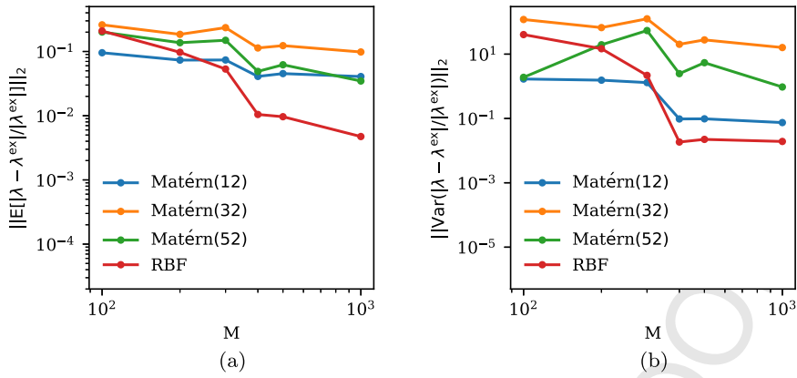
Fig. 3. Convergence comparison using different kernels. The L^2 -norm of the expectation and the variance of the relative error are shown. Here, \lambda^{ex} \in \mathbb{R}^N with N = 6 indicates the exact solution of MED taken from untrained subset of the data set. The statistics are performed over 2000 testing points.
