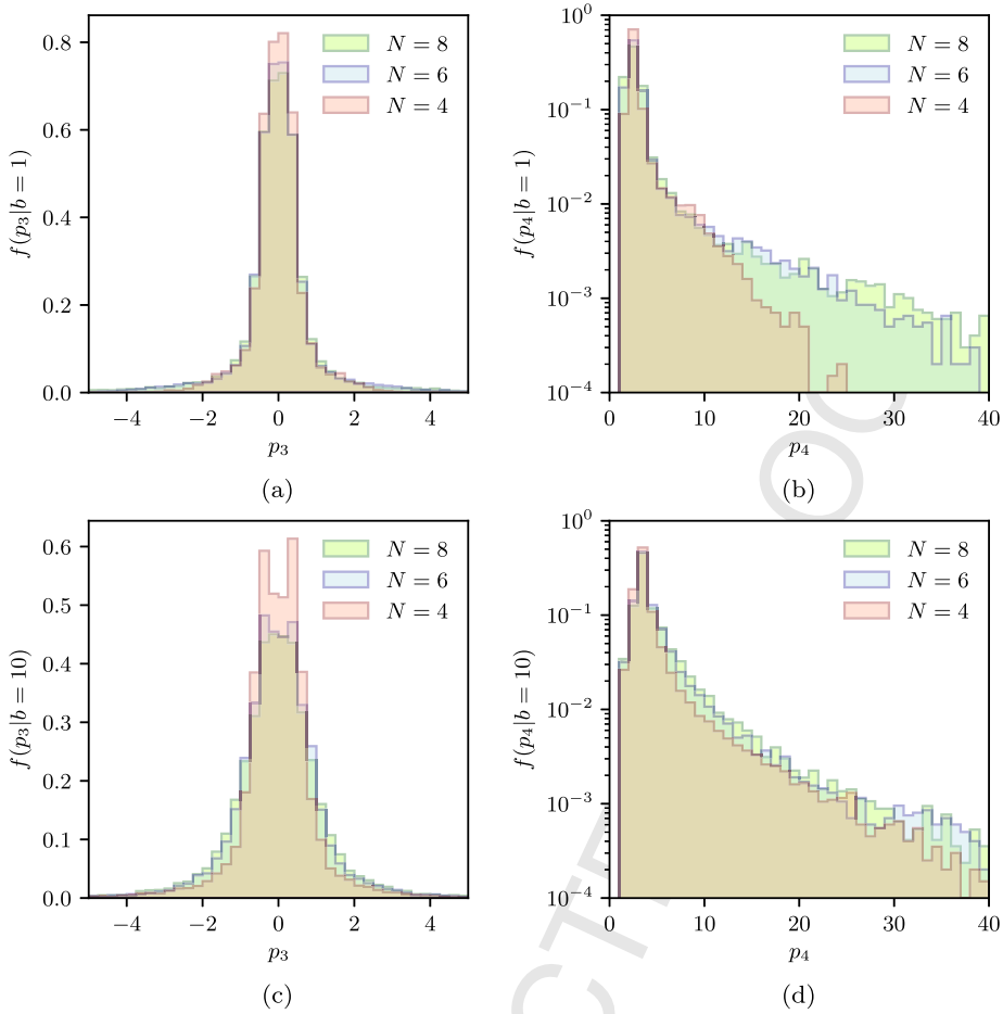
Fig. 1. Probability density function of the moments p_3 and p_4 obtained from 10^4 data points using Algorithm 2. The sample space \Lambda = [-b, b]^N for the Lagrange multipliers varies with N \in \{4, 6, 8\} and b \in \{1, 10\} .
