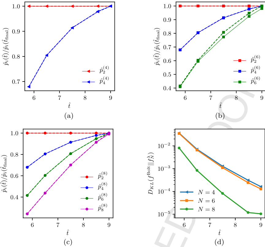
Fig. 14. Relaxation of standardized moments \hat{p}^{(N)} \in \mathbb{R}^N obtained from exact solution of the Boltzmann equation and devised MED estimation f_N^\lambda with N \in \{4, 6, 8\} depicted by dashed and solid lines, respectively, together with the KL divergence between solutions.
