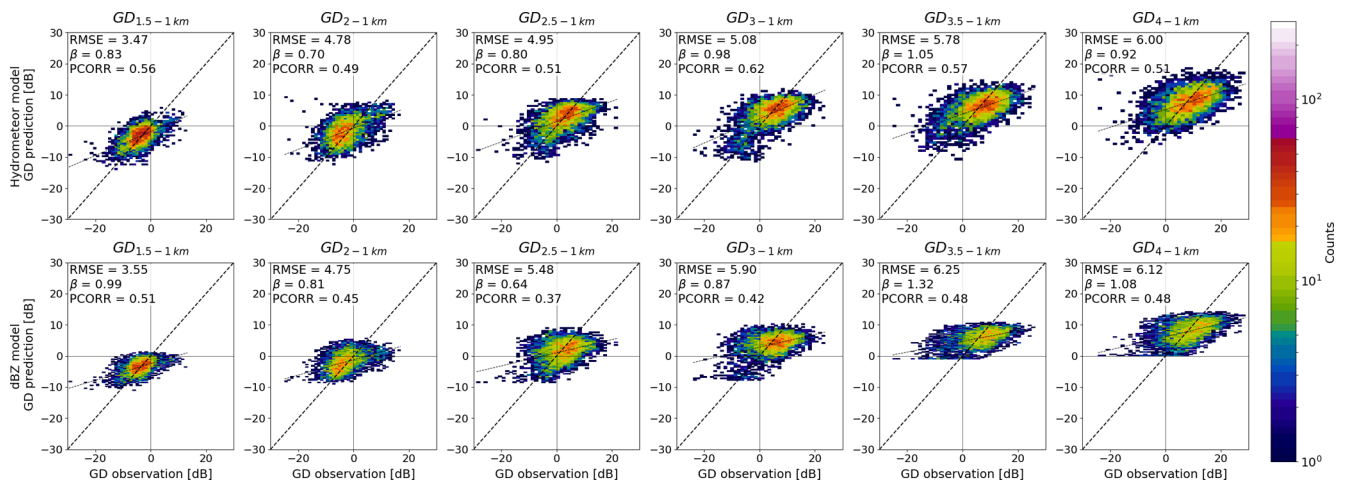
Figure 5. The 2-D histograms for observed ( x axes) and predicted ( y axes) GD for the HC + dBZ models (top row) and dBZ-only models (bottom row) trained with data starting from higher altitude levels and aloft (columns). The number of points in each bin is indicated in colour.
