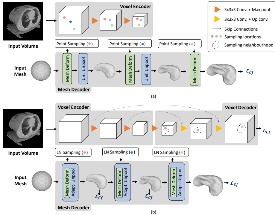
Fig. 1. Architectures (a) The Pixel2Mesh-3D architecture, a straightforward extension of [20], uses a surface decoder but no voxel decoder. (b) By contrast, our Voxel2Mesh architecture takes as input an image and spherical mesh. They are jointly encoded and then decoded into cubes and meshes of increasing resolution. At each mesh decoding stage, the decoder first receives as input the current mesh and a set of features sampled from the cube of corresponding resolution. Then the mesh is deformed and refined non-uniformly by adding vertices only where they are needed.
