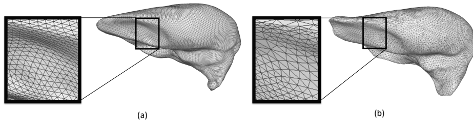
Fig. 3. Levels of resolution. (a) Pixel2Mesh-3D result (10422 vertices). (b) Voxel2Mesh result (7498 vertices). With our adaptive unpooling, we obtain better results with fewer vertices.
